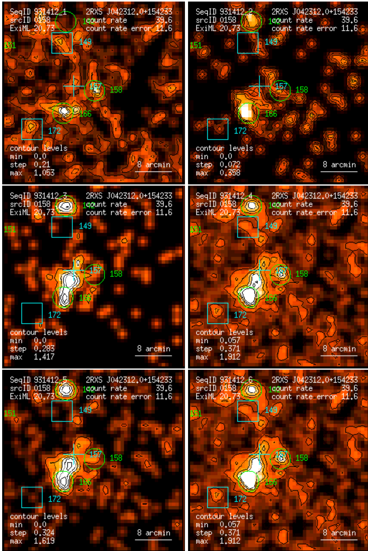
Figure 158: RASS 931412: detection 0158: band rate images, Gaussian filter: (1) PSPC channels 11 – 41, (2) 52 – 90, (3) 91 – 201, (4) 11 – 235, (5) 52 – 201, (6) 11 – 201. Broad band rates in counts/ks. Band rate contour levels in counts/ks/arcmin 2 .
