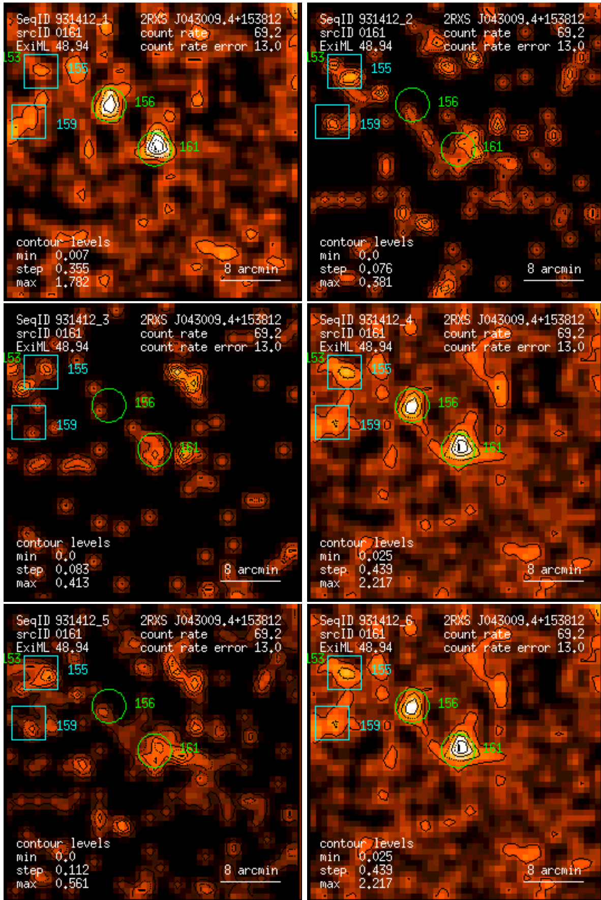
Figure 161: RASS 931412: detection 0161: band rate images, Gaussian filter: (1) PSPC channels 11 – 41, (2) 52 – 90, (3) 91 – 201, (4) 11 – 235, (5) 52 – 201, (6) 11 – 201. Broad band rates in counts/ks. Band rate contour levels in counts/ks/arcmin 2 .
