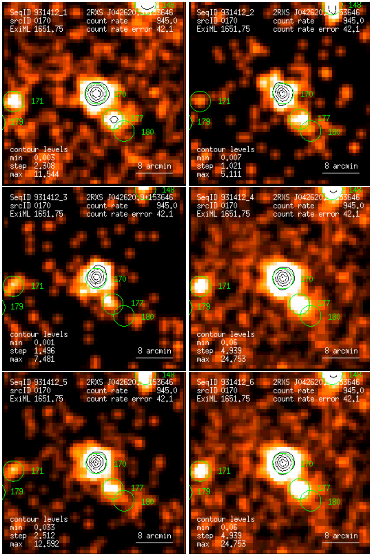
Figure 170: RASS 931412: detection 0170: band rate images, Gaussian filter: (1) PSPC channels 11 – 41, (2) 52 – 90, (3) 91 – 201, (4) 11 – 235, (5) 52 – 201, (6) 11 – 201. Broad band rates in counts/ks. Band rate contour levels in counts/ks/arcmin 2 .
