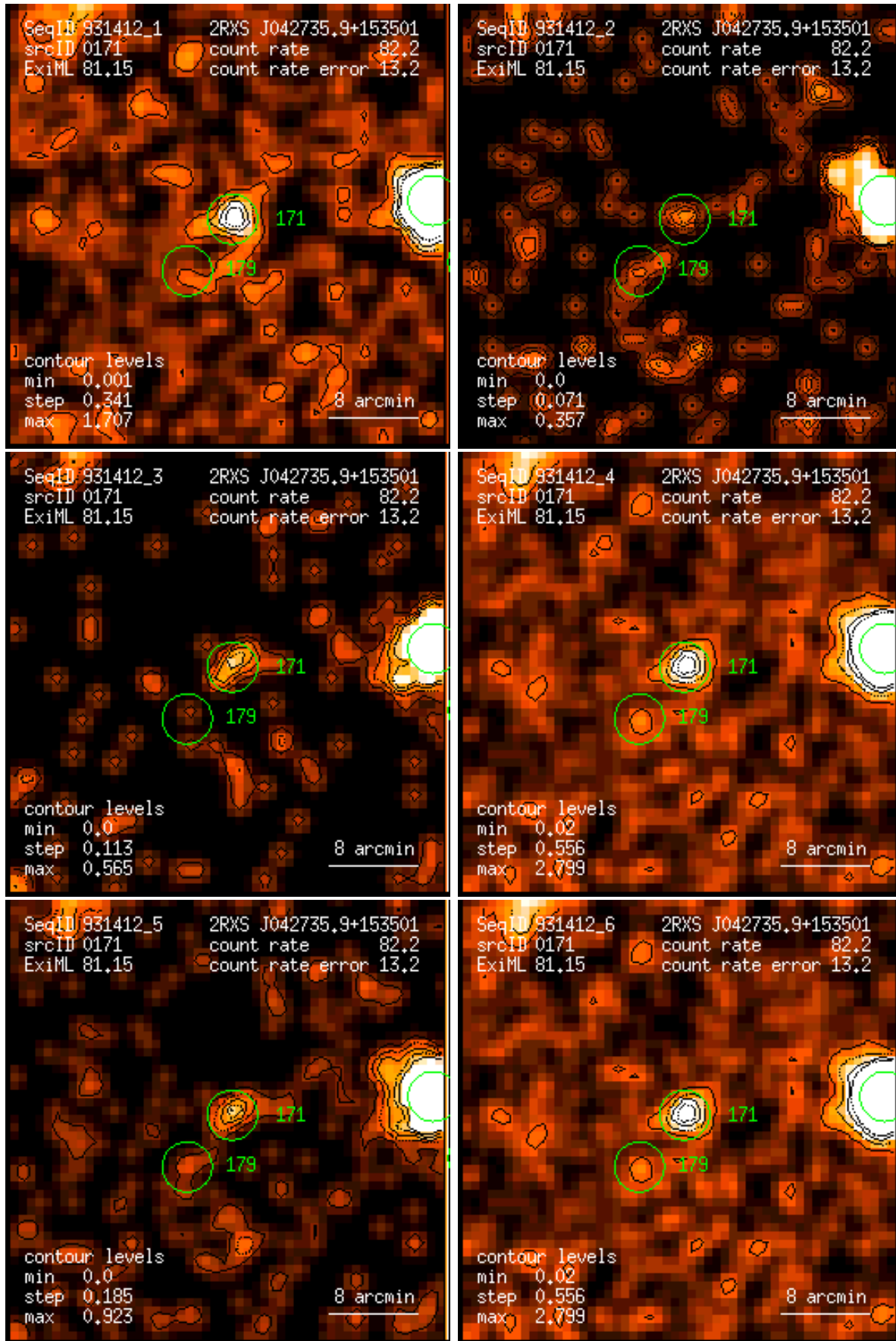
Figure 171: RASS 931412: detection 0171: band rate images, Gaussian filter: (1) PSPC channels 11 – 41, (2) 52 – 90, (3) 91 – 201, (4) 11 – 235, (5) 52 – 201, (6) 11 – 201. Broad band rates in counts/ks. Band rate contour levels in counts/ks/arcmin 2 .
