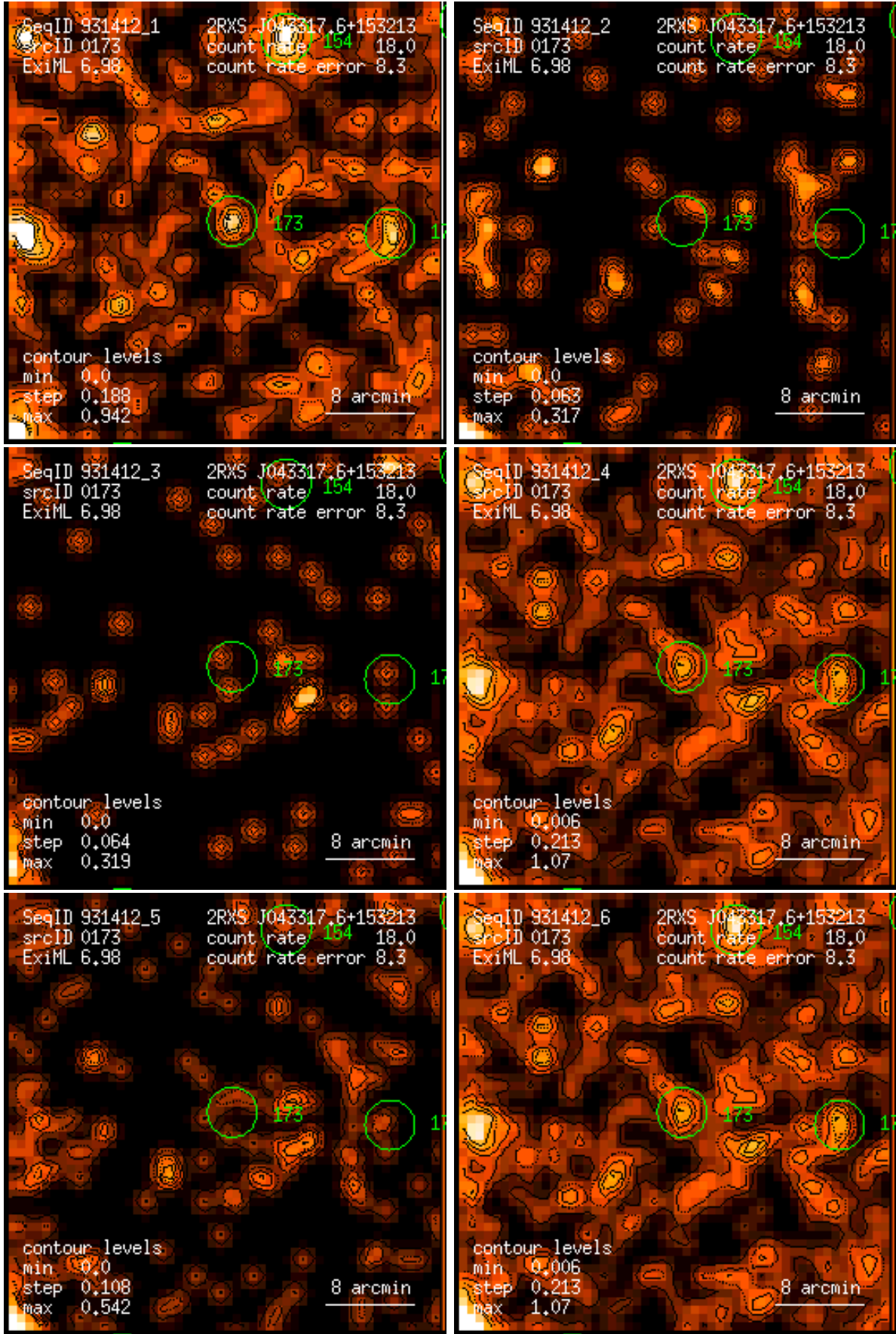
Figure 173: RASS 931412: detection 0173: band rate images, Gaussian filter: (1) PSPC channels 11 – 41, (2) 52 – 90, (3) 91 – 201, (4) 11 – 235, (5) 52 – 201, (6) 11 – 201. Broad band rates in counts/ks. Band rate contour levels in counts/ks/arcmin 2 .
