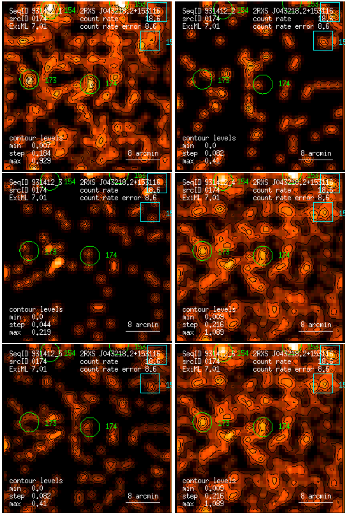
Figure 174: RASS 931412: detection 0174: band rate images, Gaussian filter: (1) PSPC channels 11 – 41, (2) 52 – 90, (3) 91 – 201, (4) 11 – 235, (5) 52 – 201, (6) 11 – 201. Broad band rates in counts/ks. Band rate contour levels in counts/ks/arcmin 2 .
