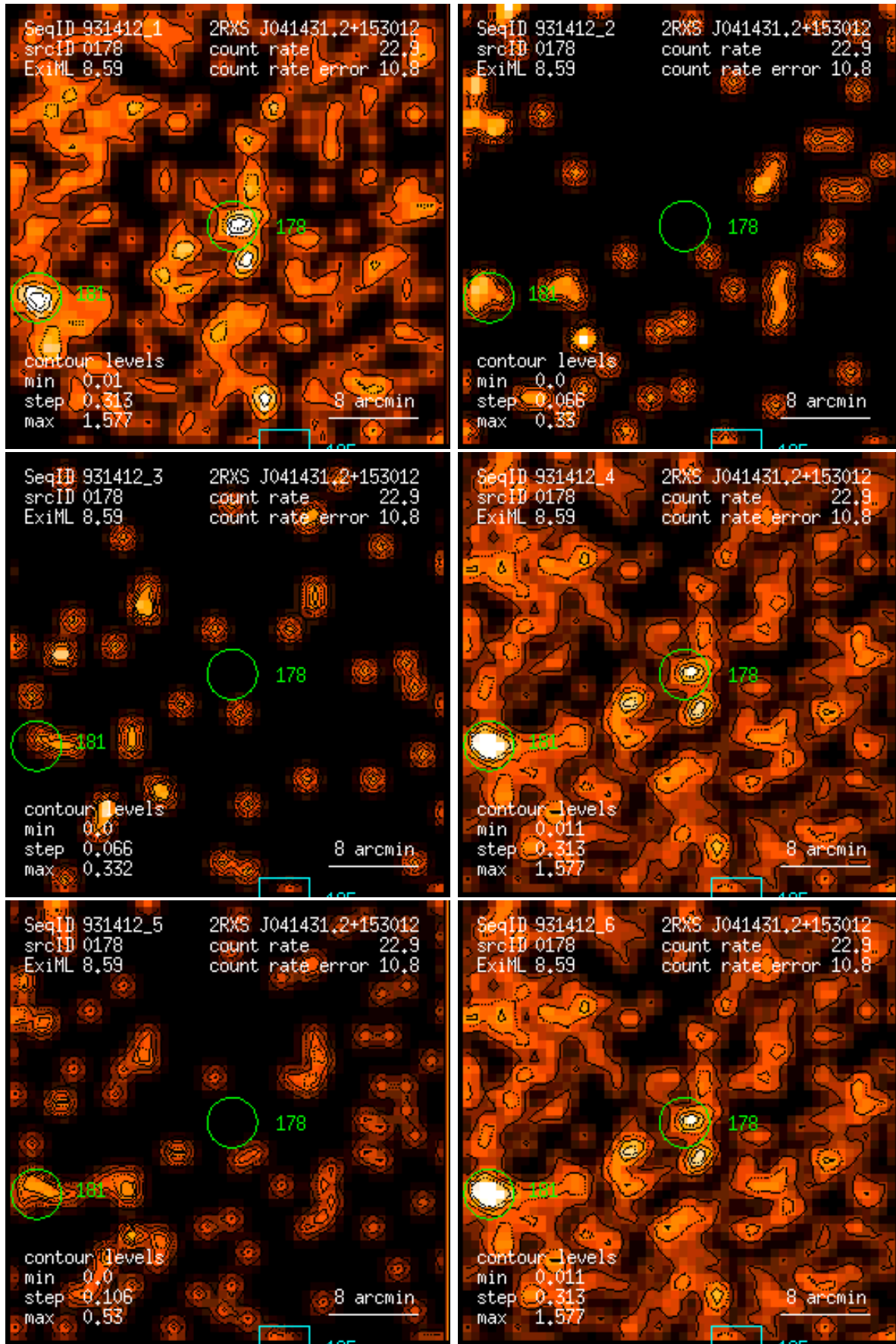
Figure 178: RASS 931412: detection 0178: band rate images, Gaussian filter: (1) PSPC channels 11 – 41, (2) 52 – 90, (3) 91 – 201, (4) 11 – 235, (5) 52 – 201, (6) 11 – 201. Broad band rates in counts/ks. Band rate contour levels in counts/ks/arcmin 2 .
