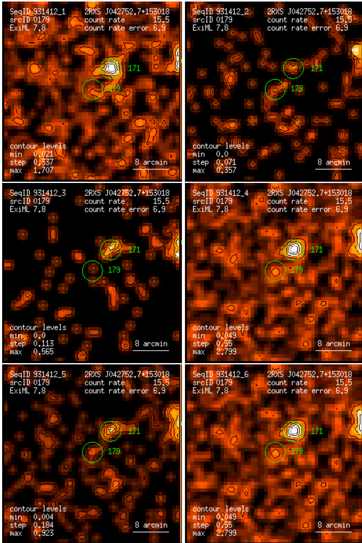
Figure 179: RASS 931412: detection 0179: band rate images, Gaussian filter: (1) PSPC channels 11 – 41, (2) 52 – 90, (3) 91 – 201, (4) 11 – 235, (5) 52 – 201, (6) 11 – 201. Broad band rates in counts/ks. Band rate contour levels in counts/ks/arcmin 2 .
