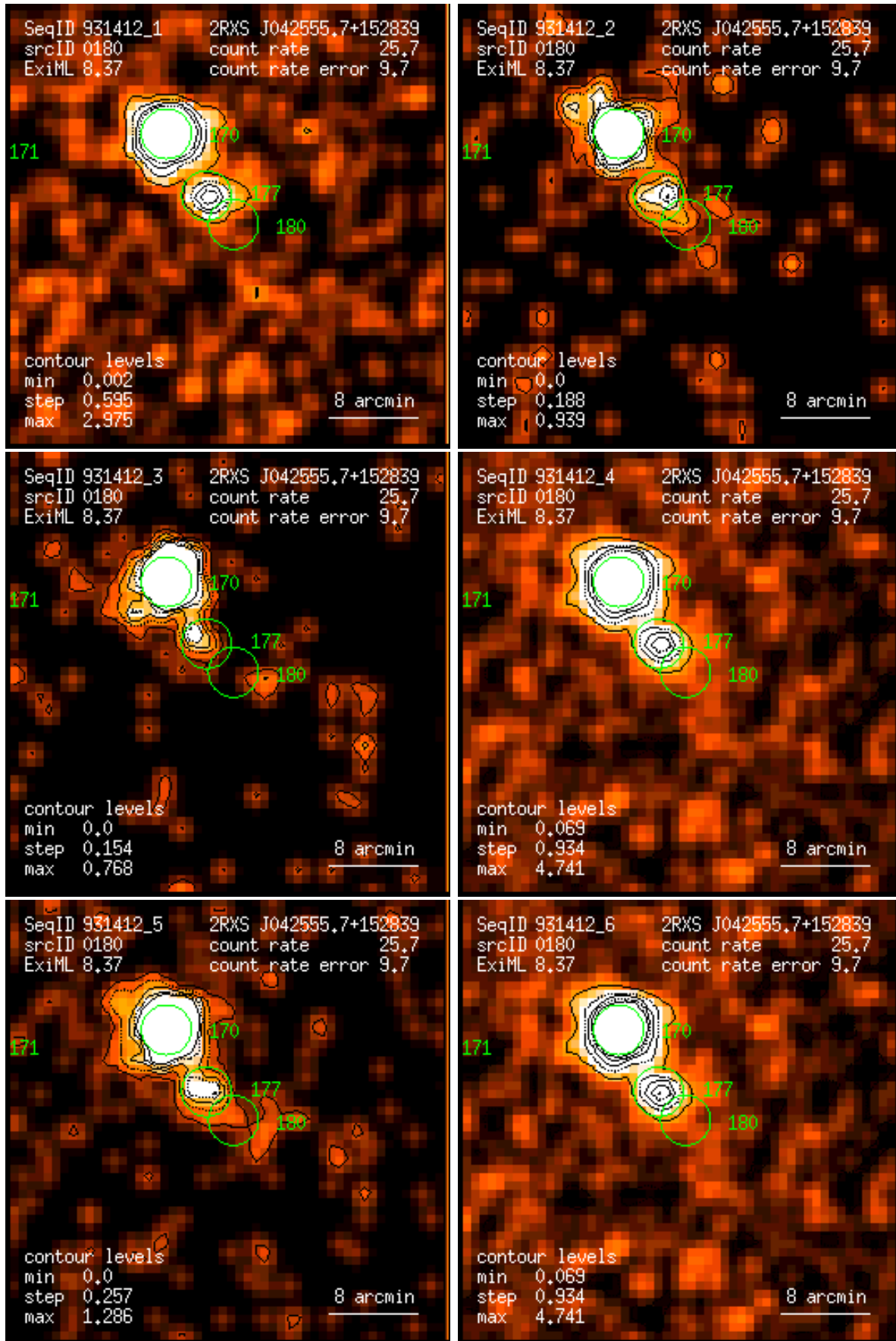
Figure 180: RASS 931412: detection 0180: band rate images, Gaussian filter: (1) PSPC channels 11 – 41, (2) 52 – 90, (3) 91 – 201, (4) 11 – 235, (5) 52 – 201, (6) 11 – 201. Broad band rates in counts/ks. Band rate contour levels in counts/ks/arcmin 2 .
