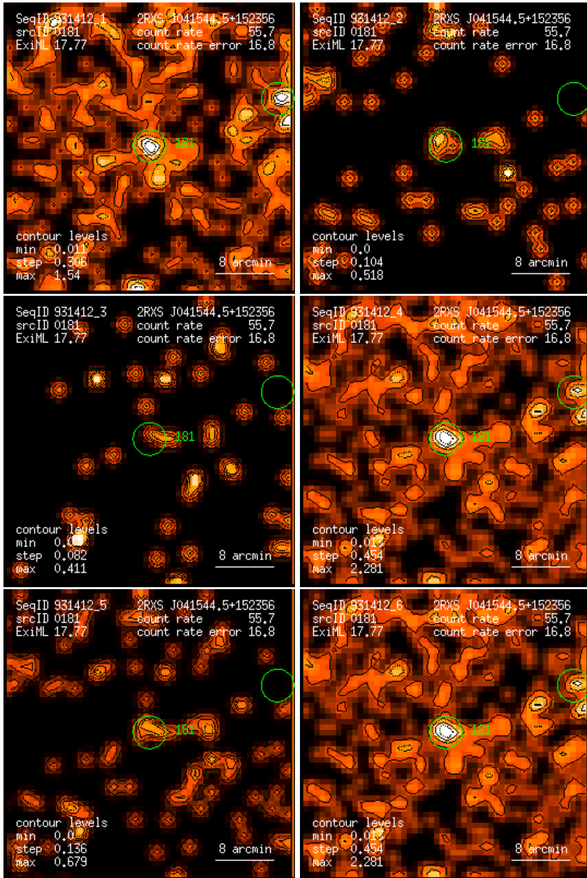
Figure 181: RASS 931412: detection 0181: band rate images, Gaussian filter: (1) PSPC channels 11 – 41, (2) 52 – 90, (3) 91 – 201, (4) 11 – 235, (5) 52 – 201, (6) 11 – 201. Broad band rates in counts/ks. Band rate contour levels in counts/ks/arcmin 2 .
