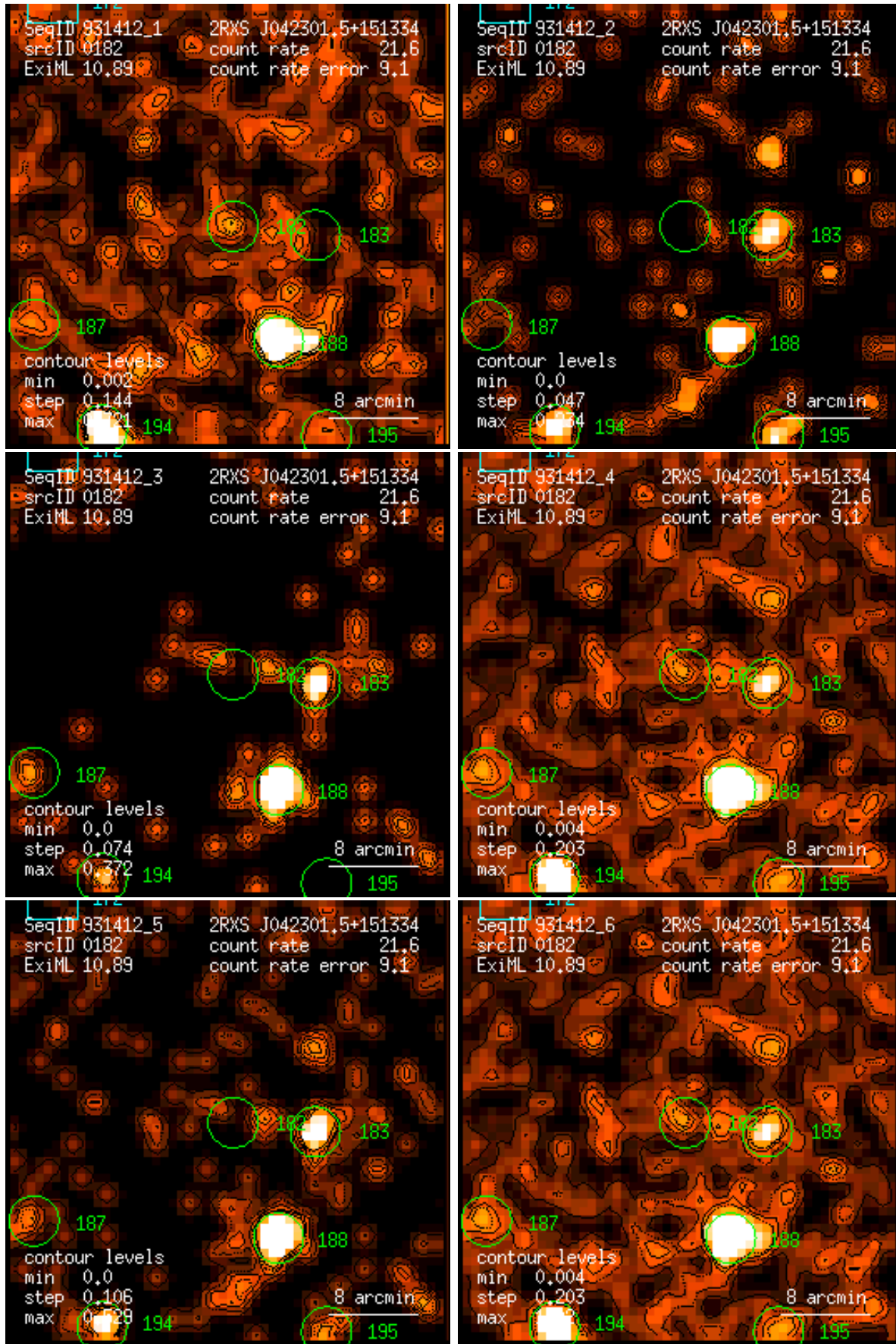
Figure 182: RASS 931412: detection 0182: band rate images, Gaussian filter: (1) PSPC channels 11 – 41, (2) 52 – 90, (3) 91 – 201, (4) 11 – 235, (5) 52 – 201, (6) 11 – 201. Broad band rates in counts/ks. Band rate contour levels in counts/ks/arcmin 2 .
