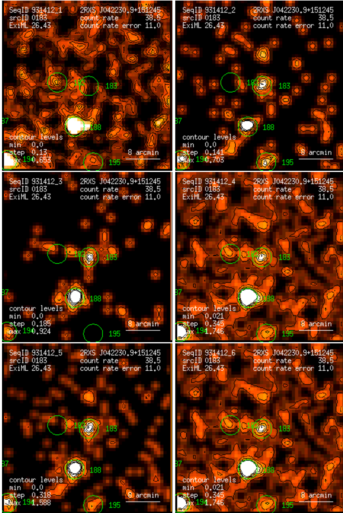
Figure 183: RASS 931412: detection 0183: band rate images, Gaussian filter: (1) PSPC channels 11 – 41, (2) 52 – 90, (3) 91 – 201, (4) 11 – 235, (5) 52 – 201, (6) 11 – 201. Broad band rates in counts/ks. Band rate contour levels in counts/ks/arcmin 2 .
