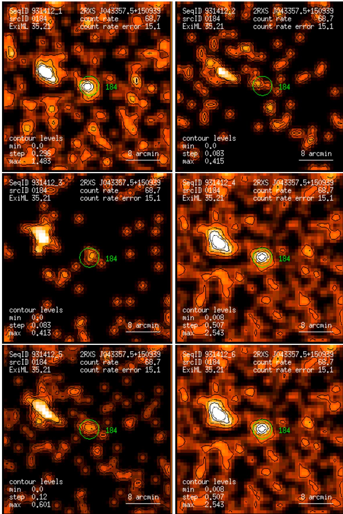
Figure 184: RASS 931412: detection 0184: band rate images, Gaussian filter: (1) PSPC channels 11 – 41, (2) 52 – 90, (3) 91 – 201, (4) 11 – 235, (5) 52 – 201, (6) 11 – 201. Broad band rates in counts/ks. Band rate contour levels in counts/ks/arcmin 2 .
