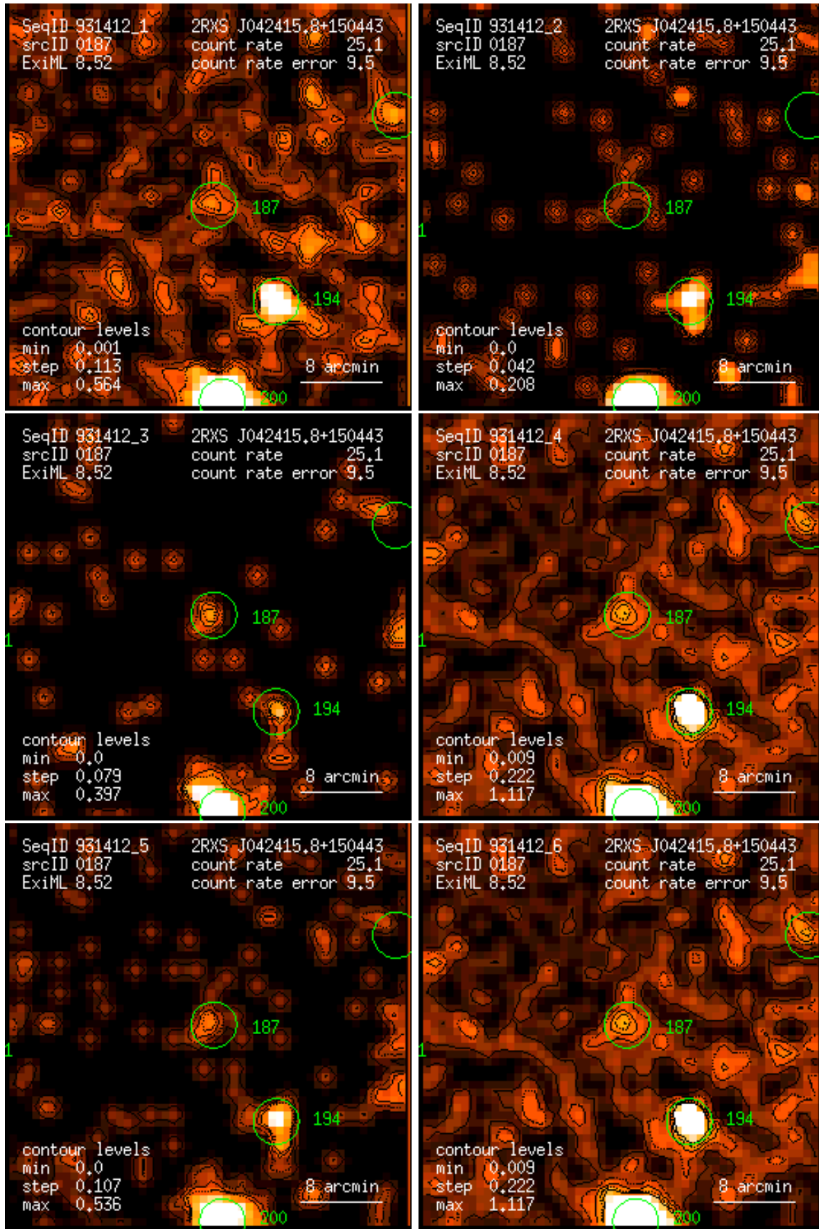
Figure 187: RASS 931412: detection 0187: band rate images, Gaussian filter: (1) PSPC channels 11 – 41, (2) 52 – 90, (3) 91 – 201, (4) 11 – 235, (5) 52 – 201, (6) 11 – 201. Broad band rates in counts/ks. Band rate contour levels in counts/ks/arcmin 2 .
