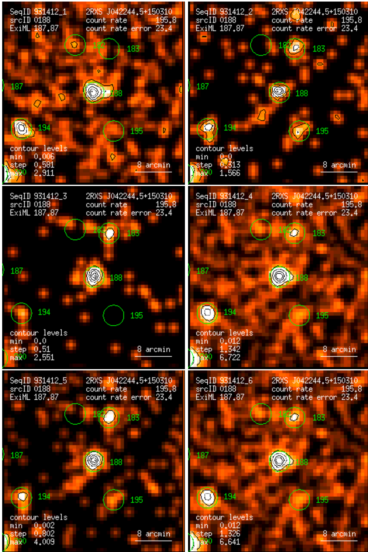
Figure 188: RASS 931412: detection 0188: band rate images, Gaussian filter: (1) PSPC channels 11 – 41, (2) 52 – 90, (3) 91 – 201, (4) 11 – 235, (5) 52 – 201, (6) 11 – 201. Broad band rates in counts/ks. Band rate contour levels in counts/ks/arcmin 2 .
