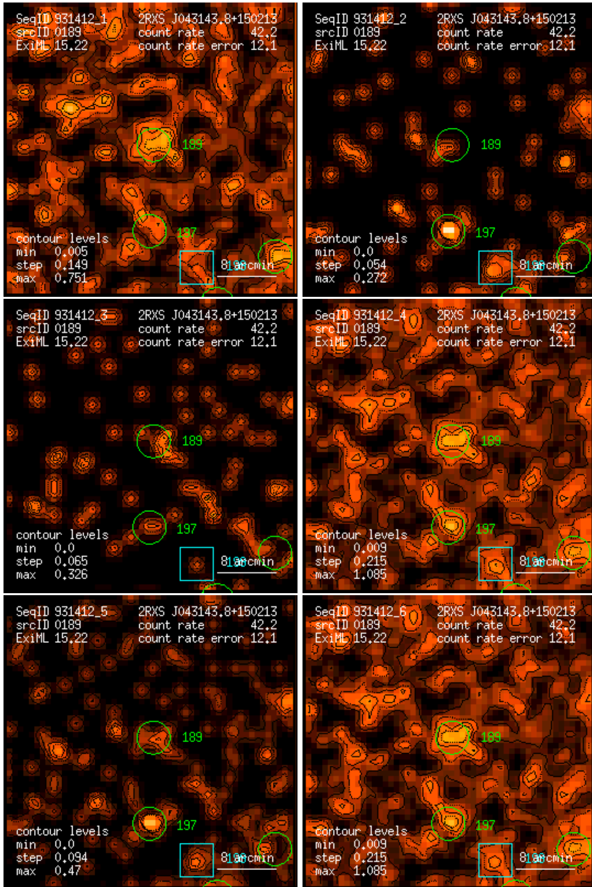
Figure 189: RASS 931412: detection 0189: band rate images, Gaussian filter: (1) PSPC channels 11 – 41, (2) 52 – 90, (3) 91 – 201, (4) 11 – 235, (5) 52 – 201, (6) 11 – 201. Broad band rates in counts/ks. Band rate contour levels in counts/ks/arcmin 2 .
