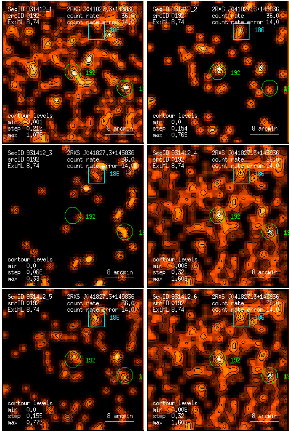
Figure 192: RASS 931412: detection 0192: band rate images, Gaussian filter: (1) PSPC channels 11 – 41, (2) 52 – 90, (3) 91 – 201, (4) 11 – 235, (5) 52 – 201, (6) 11 – 201. Broad band rates in counts/ks. Band rate contour levels in counts/ks/arcmin 2 .
