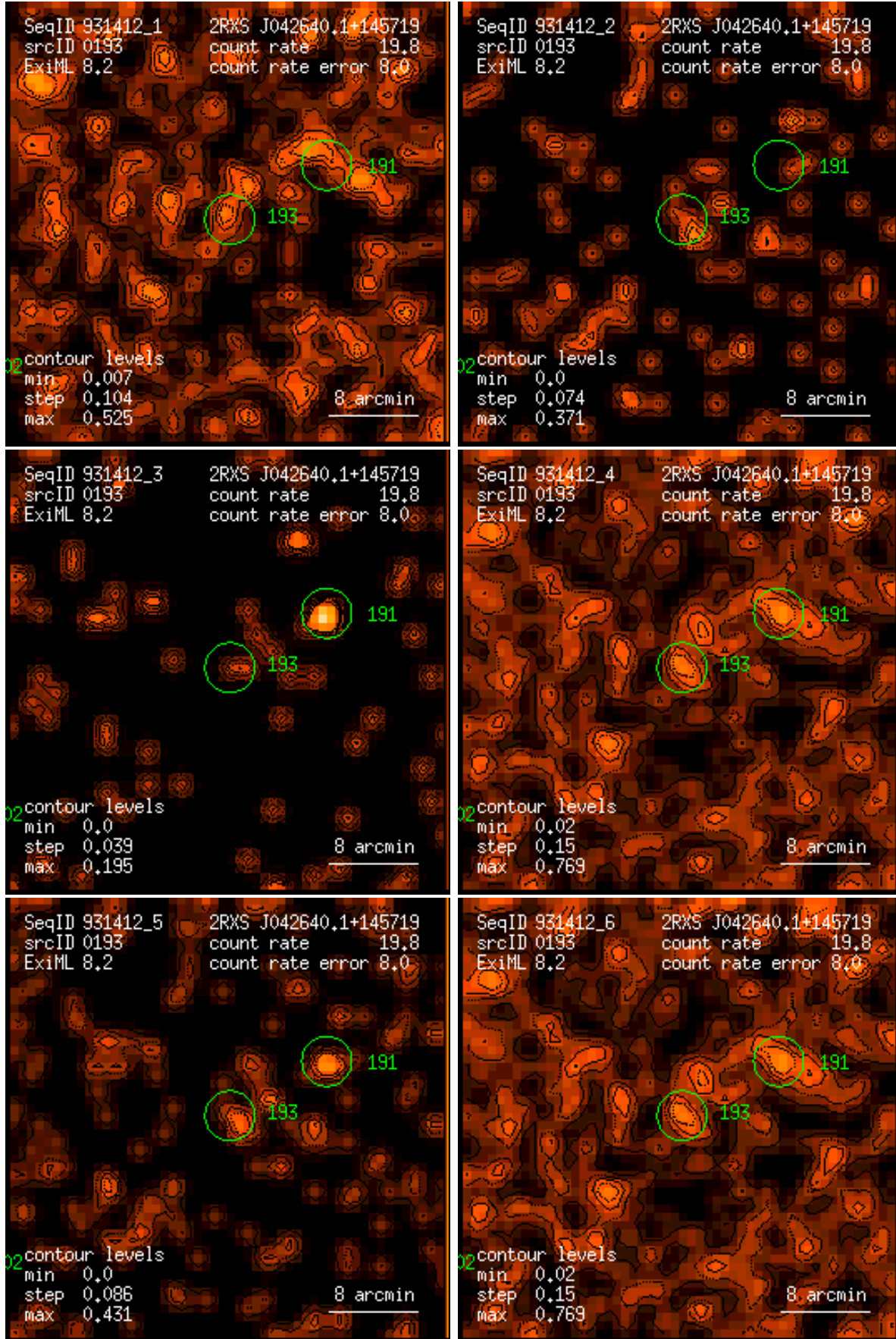
Figure 193: RASS 931412: detection 0193: band rate images, Gaussian filter: (1) PSPC channels 11 – 41, (2) 52 – 90, (3) 91 – 201, (4) 11 – 235, (5) 52 – 201, (6) 11 – 201. Broad band rates in counts/ks. Band rate contour levels in counts/ks/arcmin 2 .
