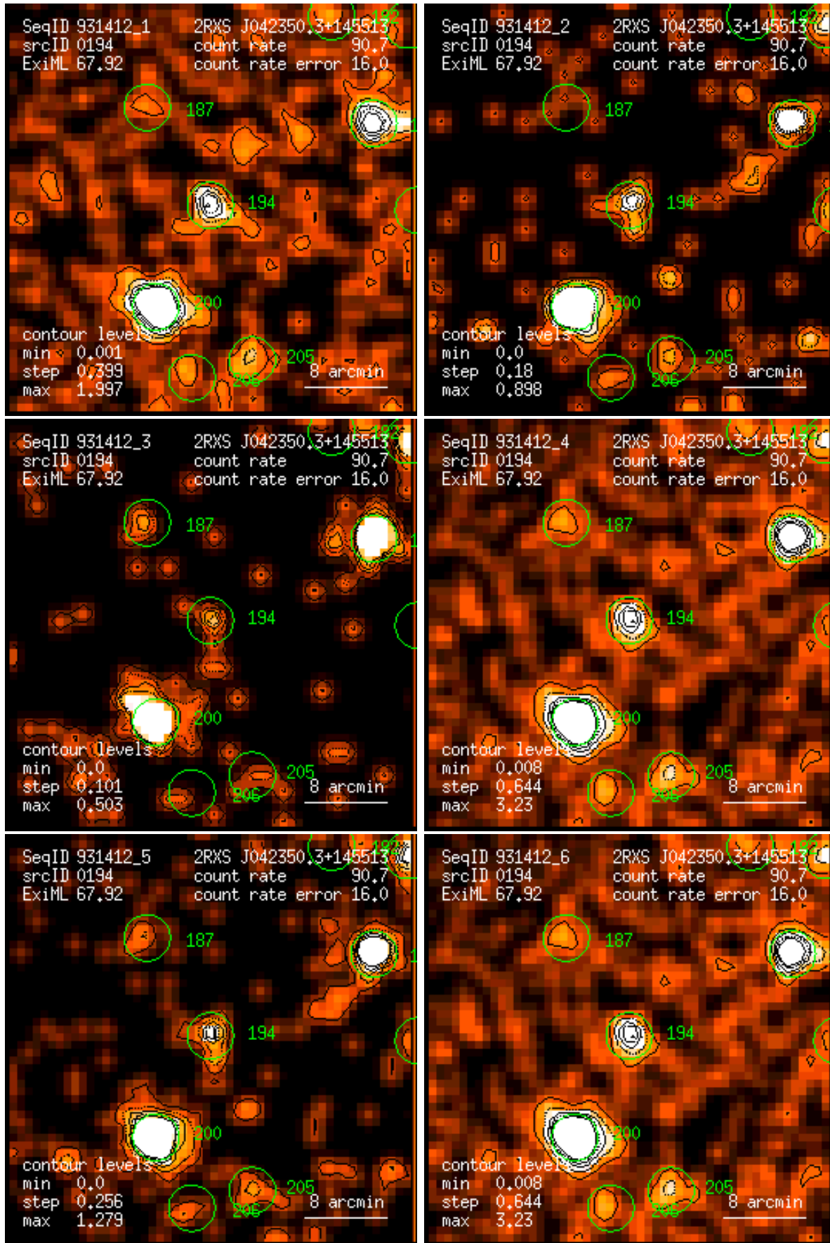
Figure 194: RASS 931412: detection 0194: band rate images, Gaussian filter: (1) PSPC channels 11 – 41, (2) 52 – 90, (3) 91 – 201, (4) 11 – 235, (5) 52 – 201, (6) 11 – 201. Broad band rates in counts/ks. Band rate contour levels in counts/ks/arcmin 2 .
