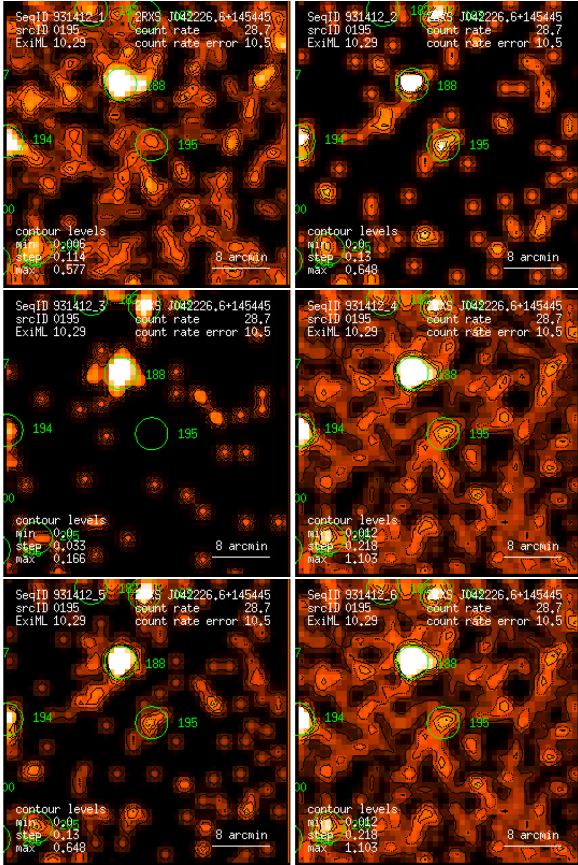
Figure 195: RASS 931412: detection 0195: band rate images, Gaussian filter: (1) PSPC channels 11 – 41, (2) 52 – 90, (3) 91 – 201, (4) 11 – 235, (5) 52 – 201, (6) 11 – 201. Broad band rates in counts/ks. Band rate contour levels in counts/ks/arcmin 2 .
