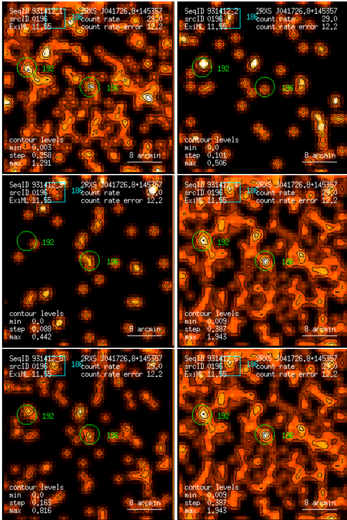
Figure 196: RASS 931412: detection 0196: band rate images, Gaussian filter: (1) PSPC channels 11 – 41, (2) 52 – 90, (3) 91 – 201, (4) 11 – 235, (5) 52 – 201, (6) 11 – 201. Broad band rates in counts/ks. Band rate contour levels in counts/ks/arcmin 2 .
