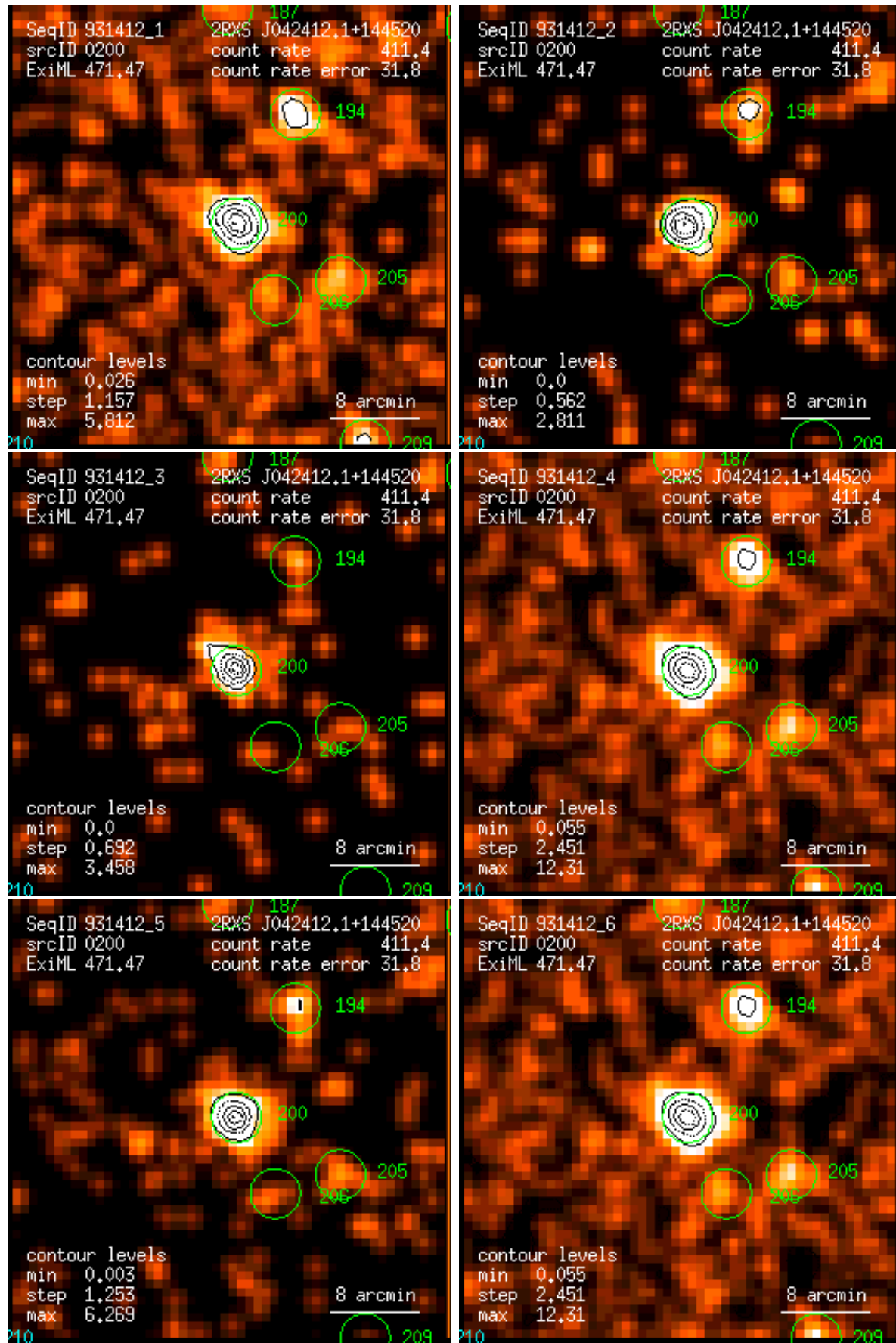
Figure 200: RASS 931412: detection 0200: band rate images, Gaussian filter: (1) PSPC channels 11 – 41, (2) 52 – 90, (3) 91 – 201, (4) 11 – 235, (5) 52 – 201, (6) 11 – 201. Broad band rates in counts/ks. Band rate contour levels in counts/ks/arcmin 2 .
