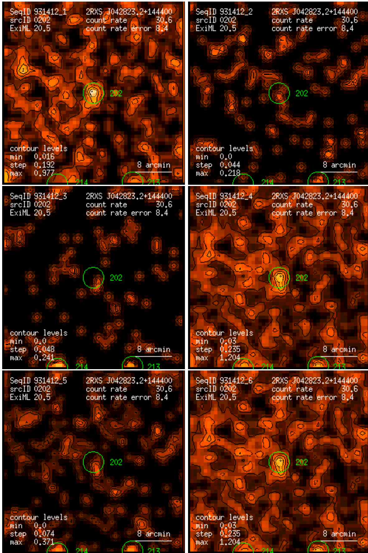
Figure 202: RASS 931412: detection 0202: band rate images, Gaussian filter: (1) PSPC channels 11 – 41, (2) 52 – 90, (3) 91 – 201, (4) 11 – 235, (5) 52 – 201, (6) 11 – 201. Broad band rates in counts/ks. Band rate contour levels in counts/ks/arcmin 2 .
