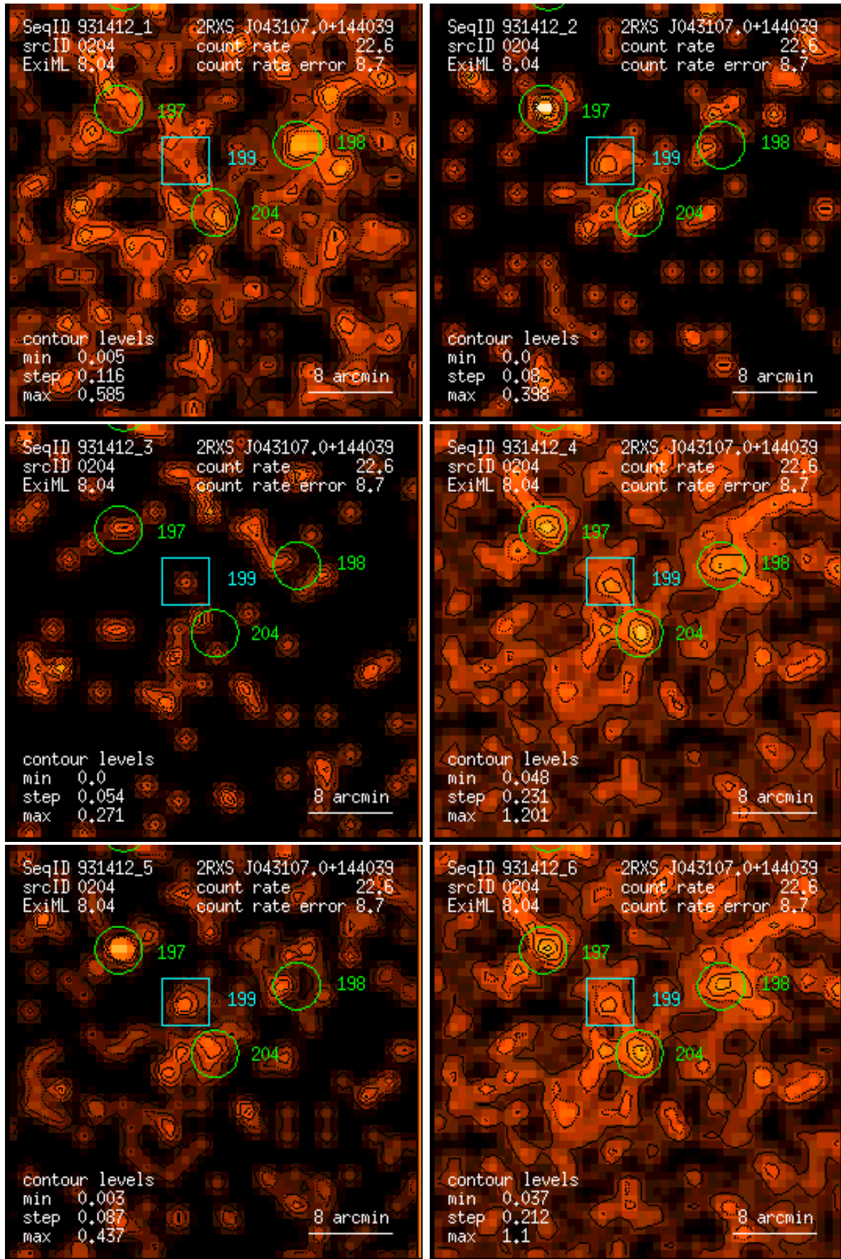
Figure 204: RASS 931412: detection 0204: band rate images, Gaussian filter: (1) PSPC channels 11 – 41, (2) 52 – 90, (3) 91 – 201, (4) 11 – 235, (5) 52 – 201, (6) 11 – 201. Broad band rates in counts/ks. Band rate contour levels in counts/ks/arcmin 2 .
