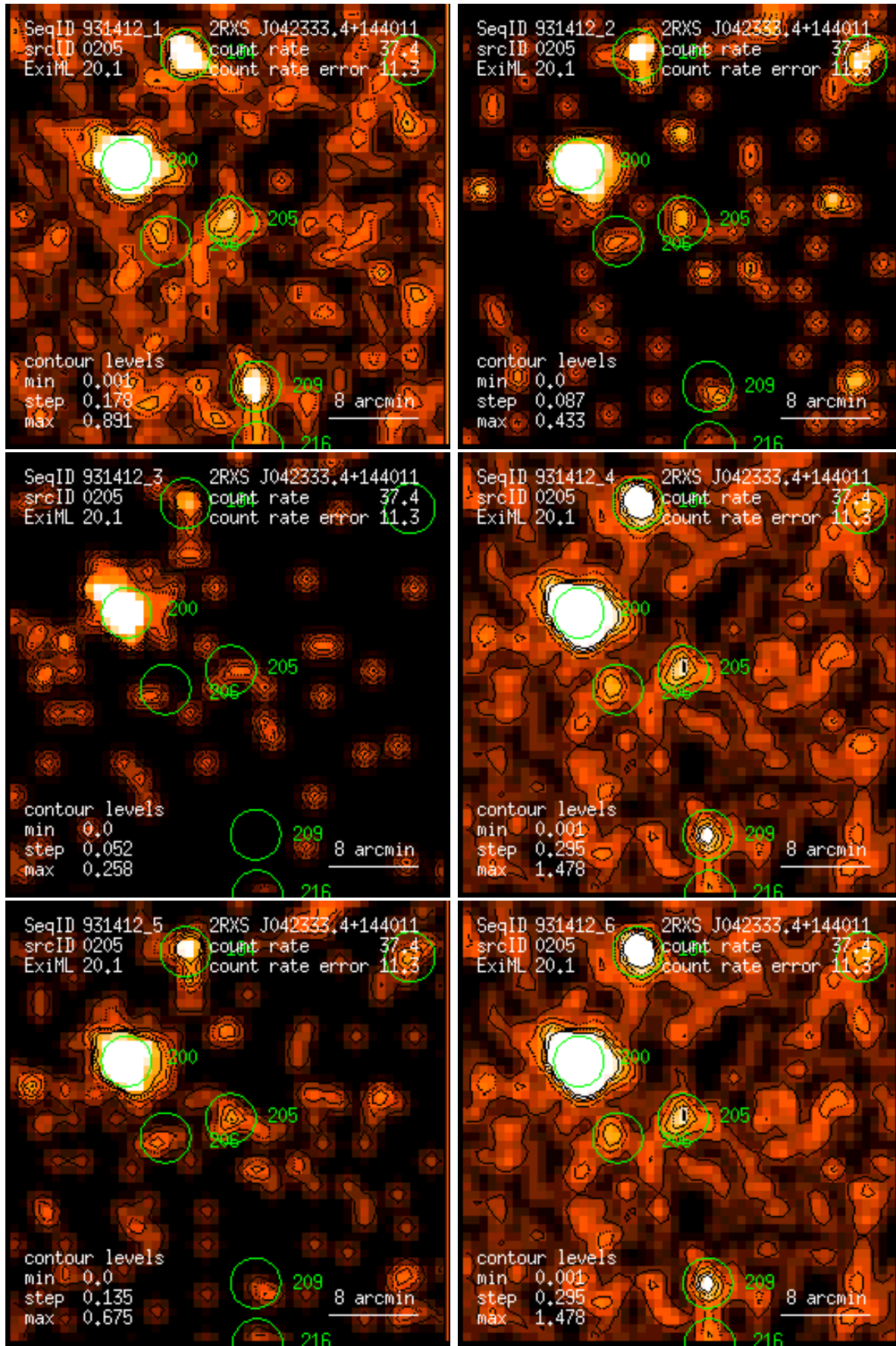
Figure 205: RASS 931412: detection 0205: band rate images, Gaussian filter: (1) PSPC channels 11 – 41, (2) 52 – 90, (3) 91 – 201, (4) 11 – 235, (5) 52 – 201, (6) 11 – 201. Broad band rates in counts/ks. Band rate contour levels in counts/ks/arcmin 2 .
