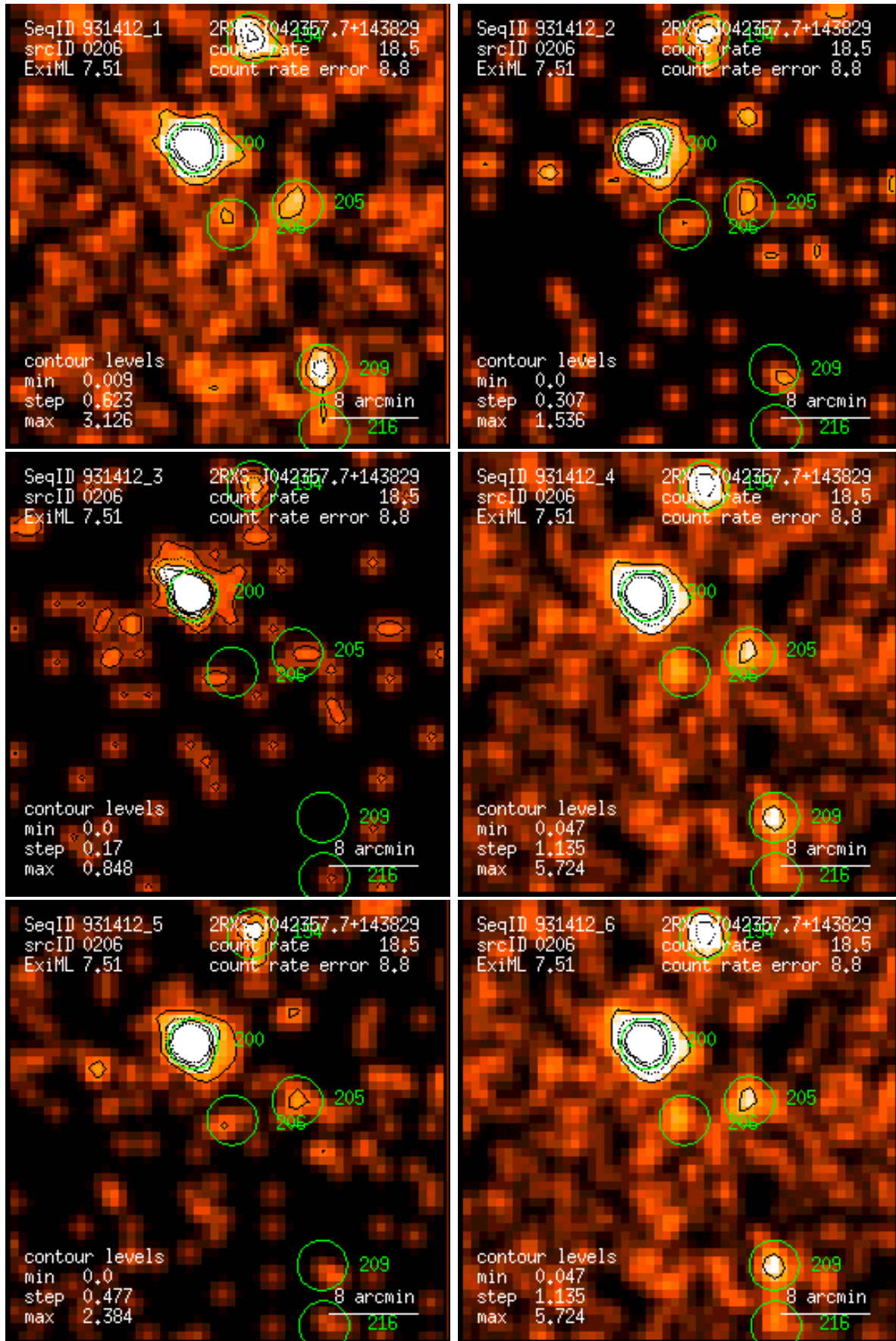
Figure 206: RASS 931412: detection 0206: band rate images, Gaussian filter: (1) PSPC channels 11 – 41, (2) 52 – 90, (3) 91 – 201, (4) 11 – 235, (5) 52 – 201, (6) 11 – 201. Broad band rates in counts/ks. Band rate contour levels in counts/ks/arcmin 2 .
