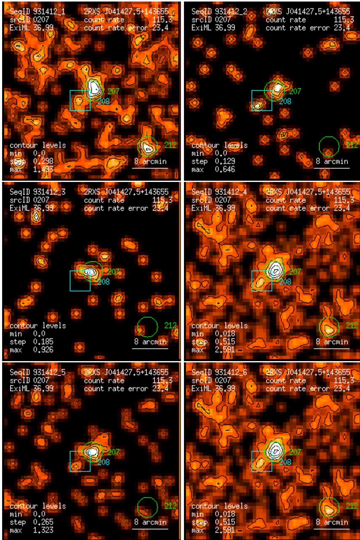
Figure 207: RASS 931412: detection 0207: band rate images, Gaussian filter: (1) PSPC channels 11 – 41, (2) 52 – 90, (3) 91 – 201, (4) 11 – 235, (5) 52 – 201, (6) 11 – 201. Broad band rates in counts/ks. Band rate contour levels in counts/ks/arcmin 2 .
