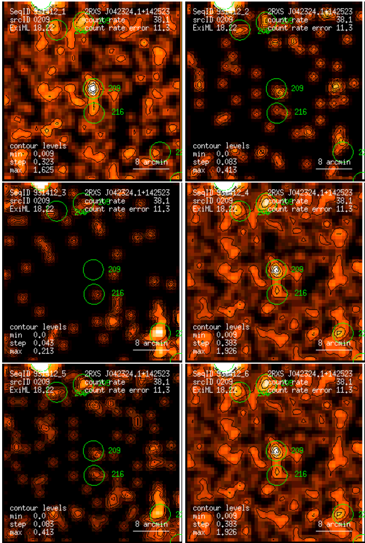
Figure 209: RASS 931412: detection 0209: band rate images, Gaussian filter: (1) PSPC channels 11 – 41, (2) 52 – 90, (3) 91 – 201, (4) 11 – 235, (5) 52 – 201, (6) 11 – 201. Broad band rates in counts/ks. Band rate contour levels in counts/ks/arcmin 2 .
