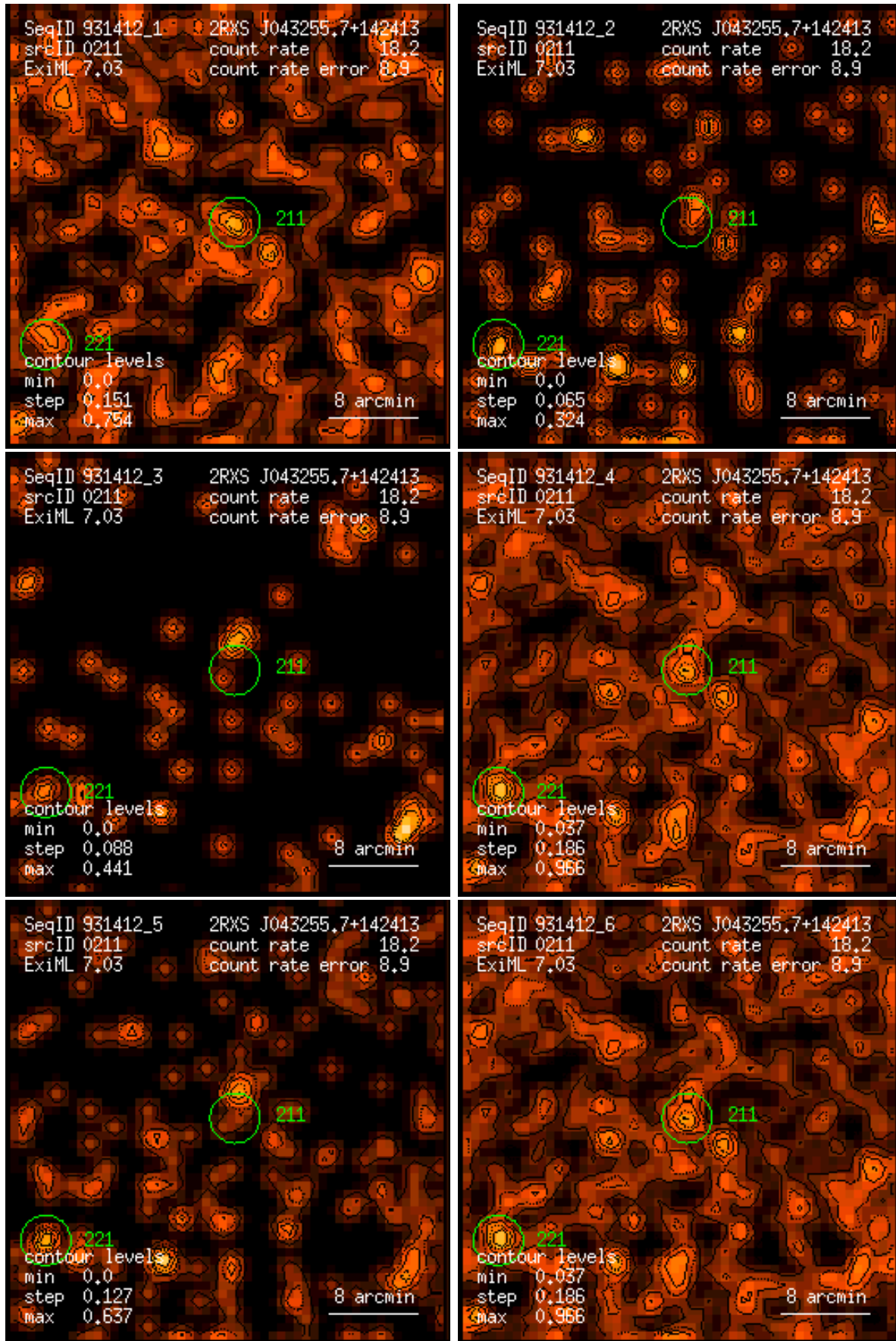
Figure 211: RASS 931412: detection 0211: band rate images, Gaussian filter: (1) PSPC channels 11 – 41, (2) 52 – 90, (3) 91 – 201, (4) 11 – 235, (5) 52 – 201, (6) 11 – 201. Broad band rates in counts/ks. Band rate contour levels in counts/ks/arcmin 2 .
