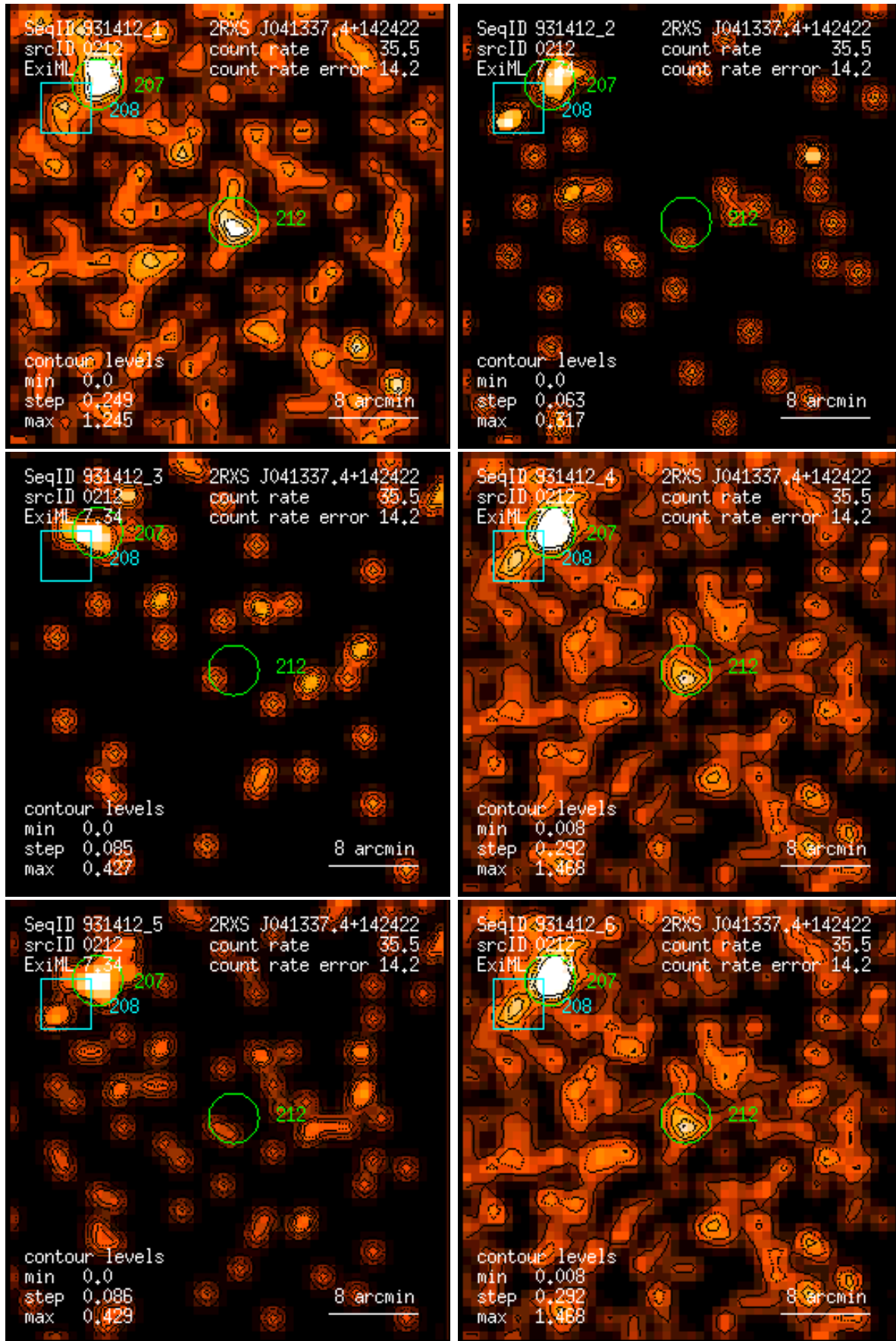
Figure 212: RASS 931412: detection 0212: band rate images, Gaussian filter: (1) PSPC channels 11 – 41, (2) 52 – 90, (3) 91 – 201, (4) 11 – 235, (5) 52 – 201, (6) 11 – 201. Broad band rates in counts/ks. Band rate contour levels in counts/ks/arcmin 2 .
