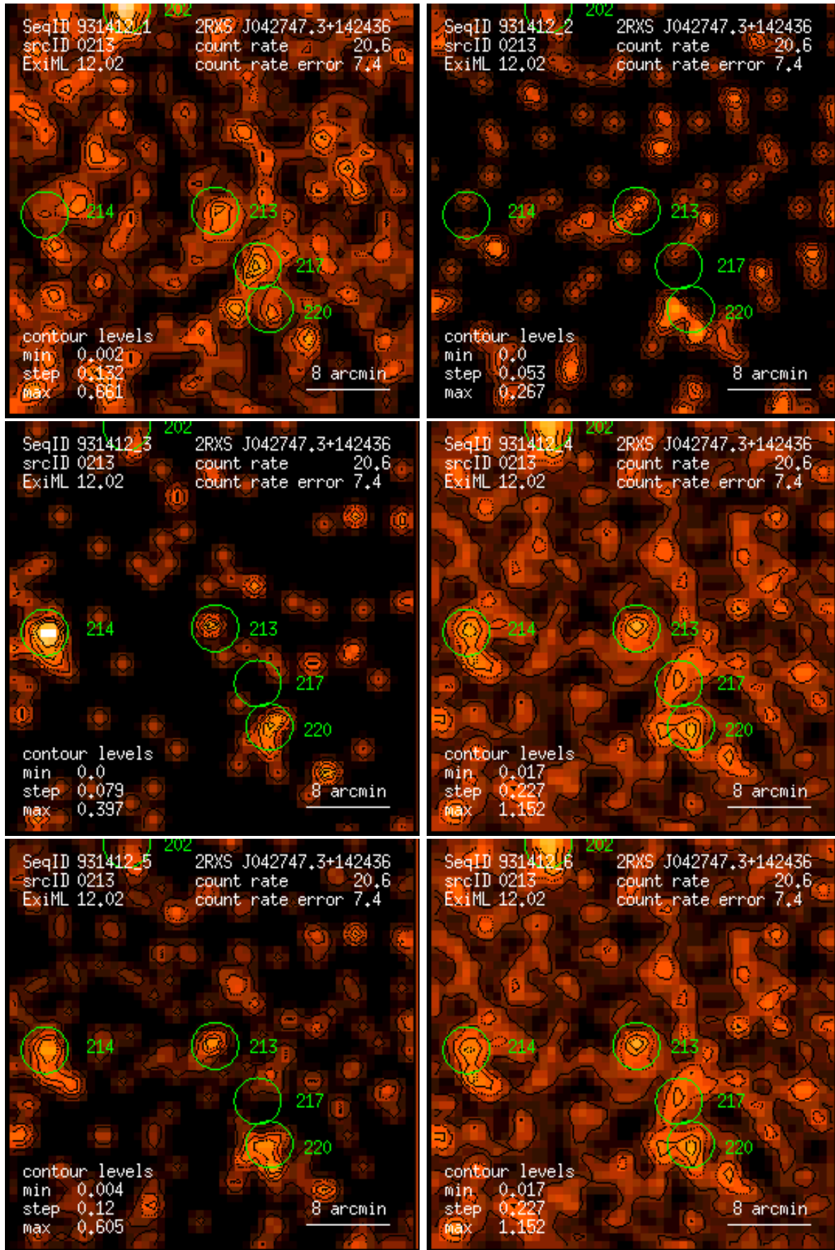
Figure 213: RASS 931412: detection 0213: band rate images, Gaussian filter: (1) PSPC channels 11 – 41, (2) 52 – 90, (3) 91 – 201, (4) 11 – 235, (5) 52 – 201, (6) 11 – 201. Broad band rates in counts/ks. Band rate contour levels in counts/ks/arcmin 2 .
