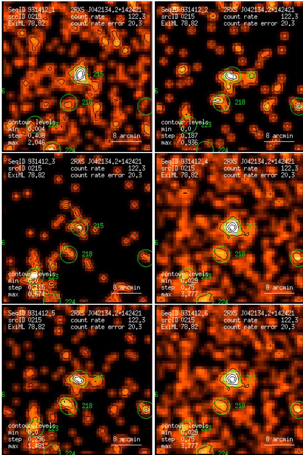
Figure 215: RASS 931412: detection 0215: band rate images, Gaussian filter: (1) PSPC channels 11 – 41, (2) 52 – 90, (3) 91 – 201, (4) 11 – 235, (5) 52 – 201, (6) 11 – 201. Broad band rates in counts/ks. Band rate contour levels in counts/ks/arcmin 2 .
