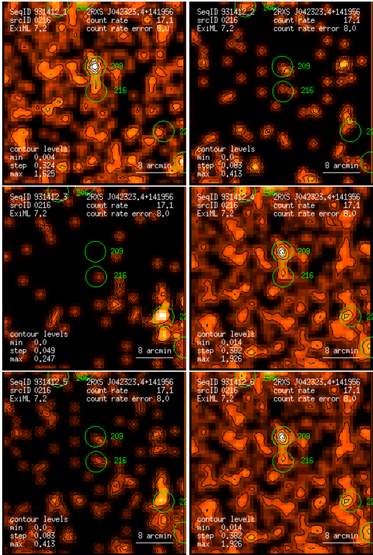
Figure 216: RASS 931412: detection 0216: band rate images, Gaussian filter: (1) PSPC channels 11 – 41, (2) 52 – 90, (3) 91 – 201, (4) 11 – 235, (5) 52 – 201, (6) 11 – 201. Broad band rates in counts/ks. Band rate contour levels in counts/ks/arcmin 2 .
