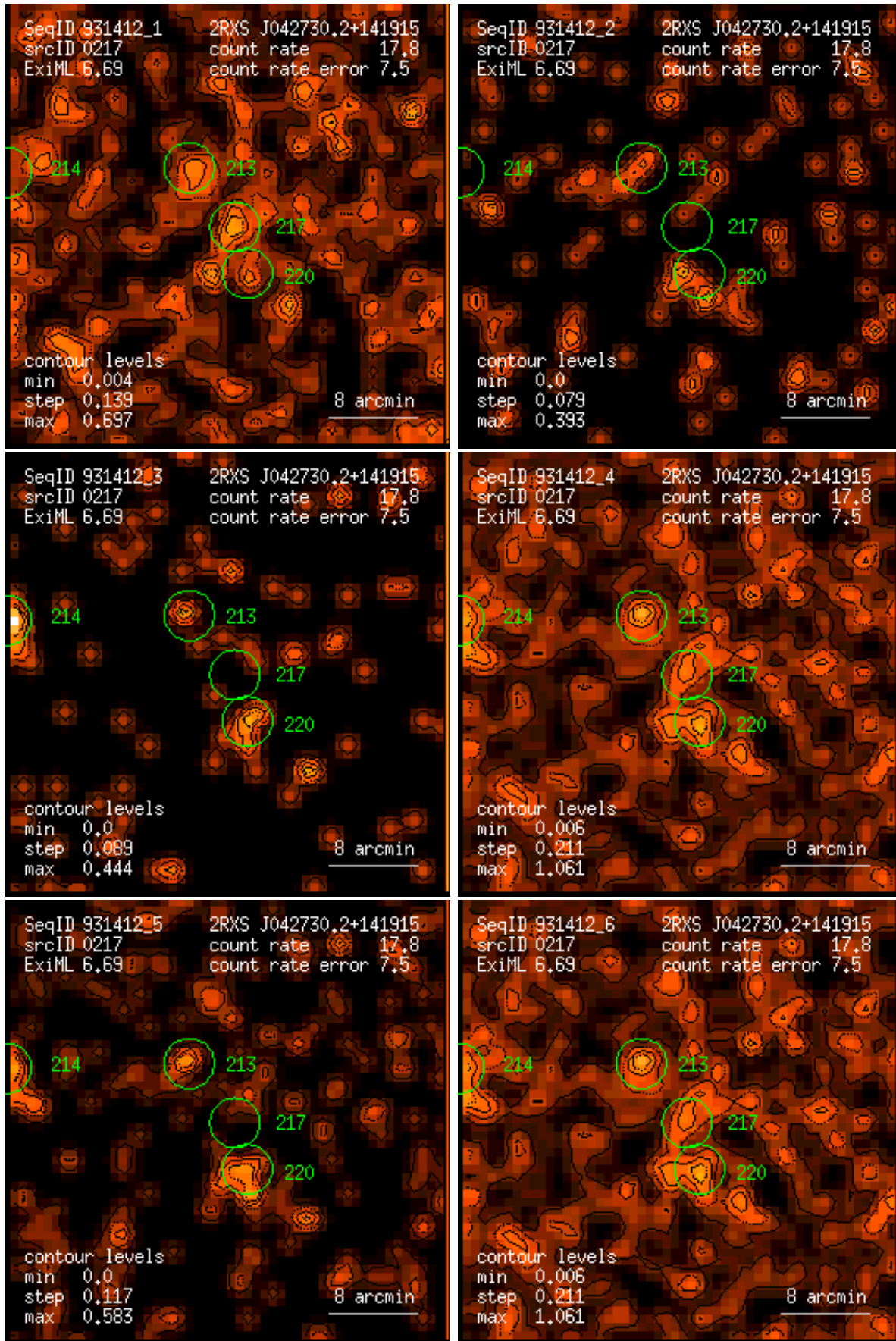
Figure 217: RASS 931412: detection 0217: band rate images, Gaussian filter: (1) PSPC channels 11 – 41, (2) 52 – 90, (3) 91 – 201, (4) 11 – 235, (5) 52 – 201, (6) 11 – 201. Broad band rates in counts/ks. Band rate contour levels in counts/ks/arcmin 2 .
