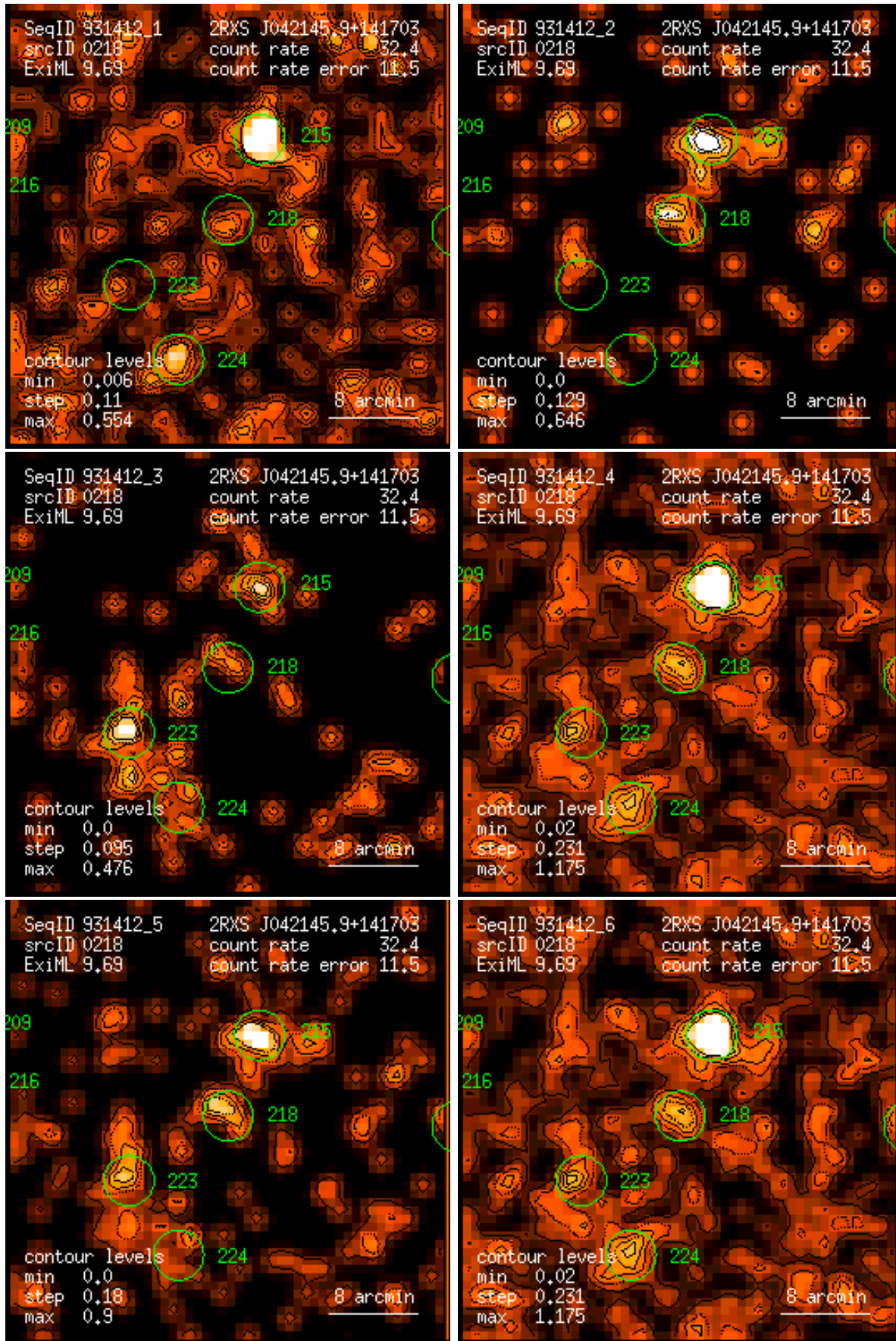
Figure 218: RASS 931412: detection 0218: band rate images, Gaussian filter: (1) PSPC channels 11 – 41, (2) 52 – 90, (3) 91 – 201, (4) 11 – 235, (5) 52 – 201, (6) 11 – 201. Broad band rates in counts/ks. Band rate contour levels in counts/ks/arcmin 2 .
