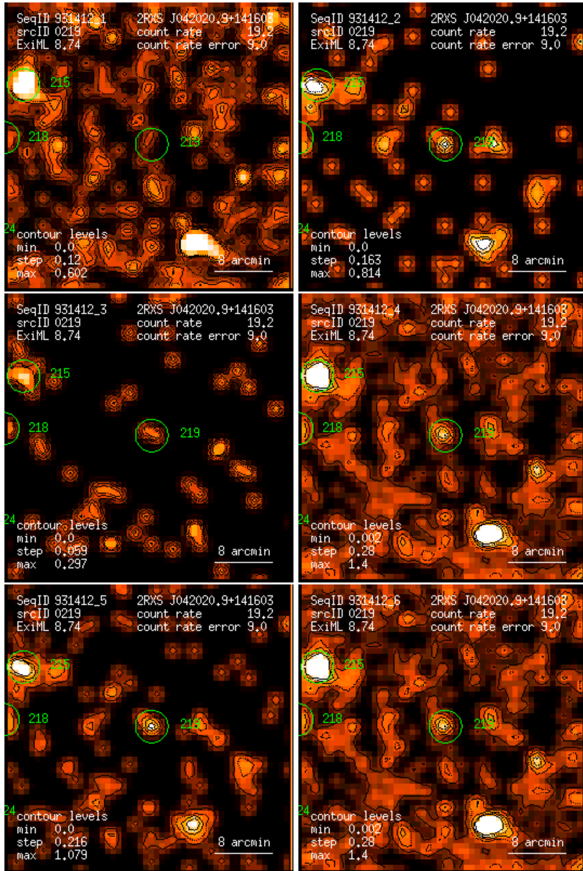
Figure 219: RASS 931412: detection 0219: band rate images, Gaussian filter: (1) PSPC channels 11 – 41, (2) 52 – 90, (3) 91 – 201, (4) 11 – 235, (5) 52 – 201, (6) 11 – 201. Broad band rates in counts/ks. Band rate contour levels in counts/ks/arcmin 2 .
