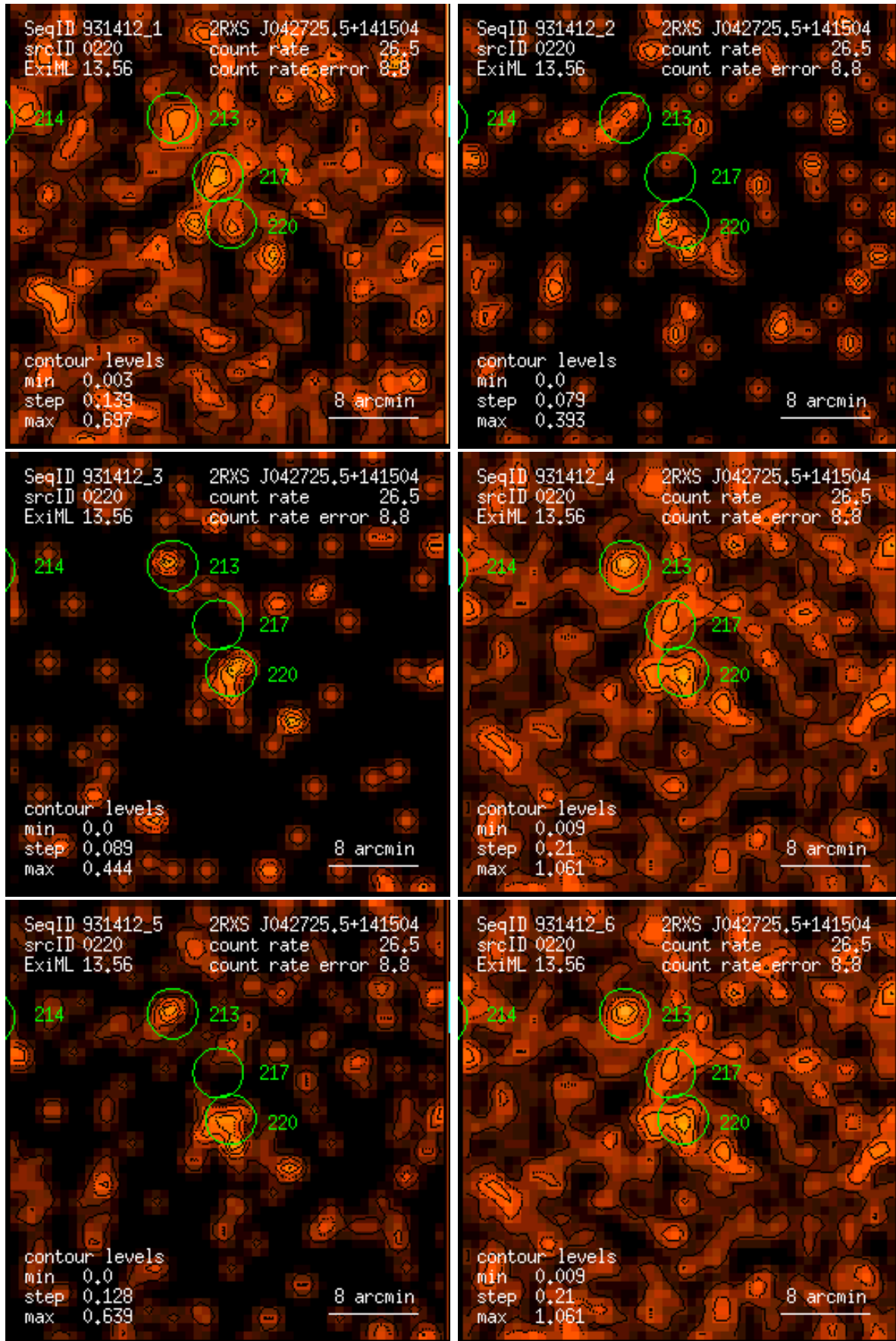
Figure 220: RASS 931412: detection 0220: band rate images, Gaussian filter: (1) PSPC channels 11 – 41, (2) 52 – 90, (3) 91 – 201, (4) 11 – 235, (5) 52 – 201, (6) 11 – 201. Broad band rates in counts/ks. Band rate contour levels in counts/ks/arcmin 2 .
