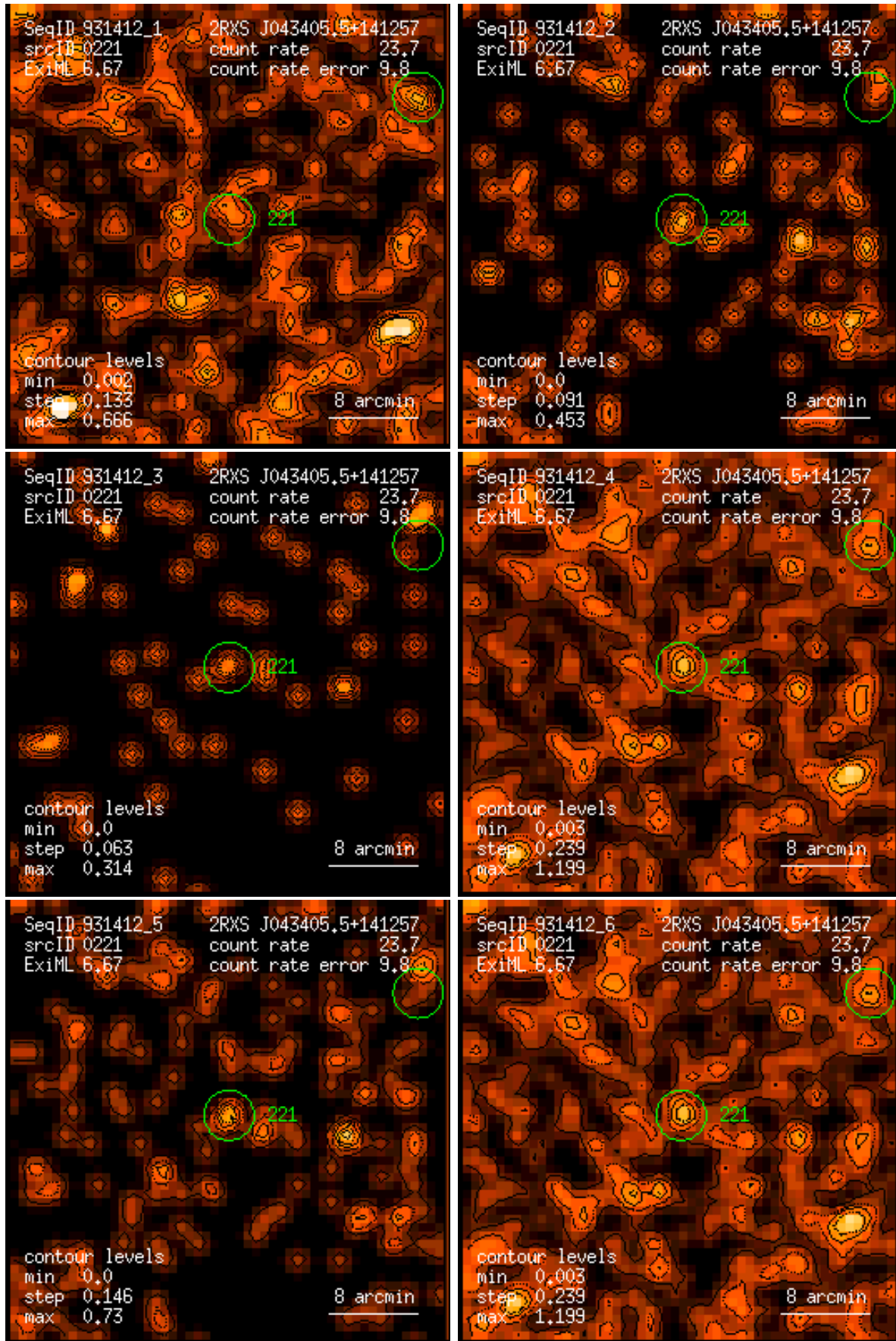
Figure 221: RASS 931412: detection 0221: band rate images, Gaussian filter: (1) PSPC channels 11 – 41, (2) 52 – 90, (3) 91 – 201, (4) 11 – 235, (5) 52 – 201, (6) 11 – 201. Broad band rates in counts/ks. Band rate contour levels in counts/ks/arcmin 2 .
