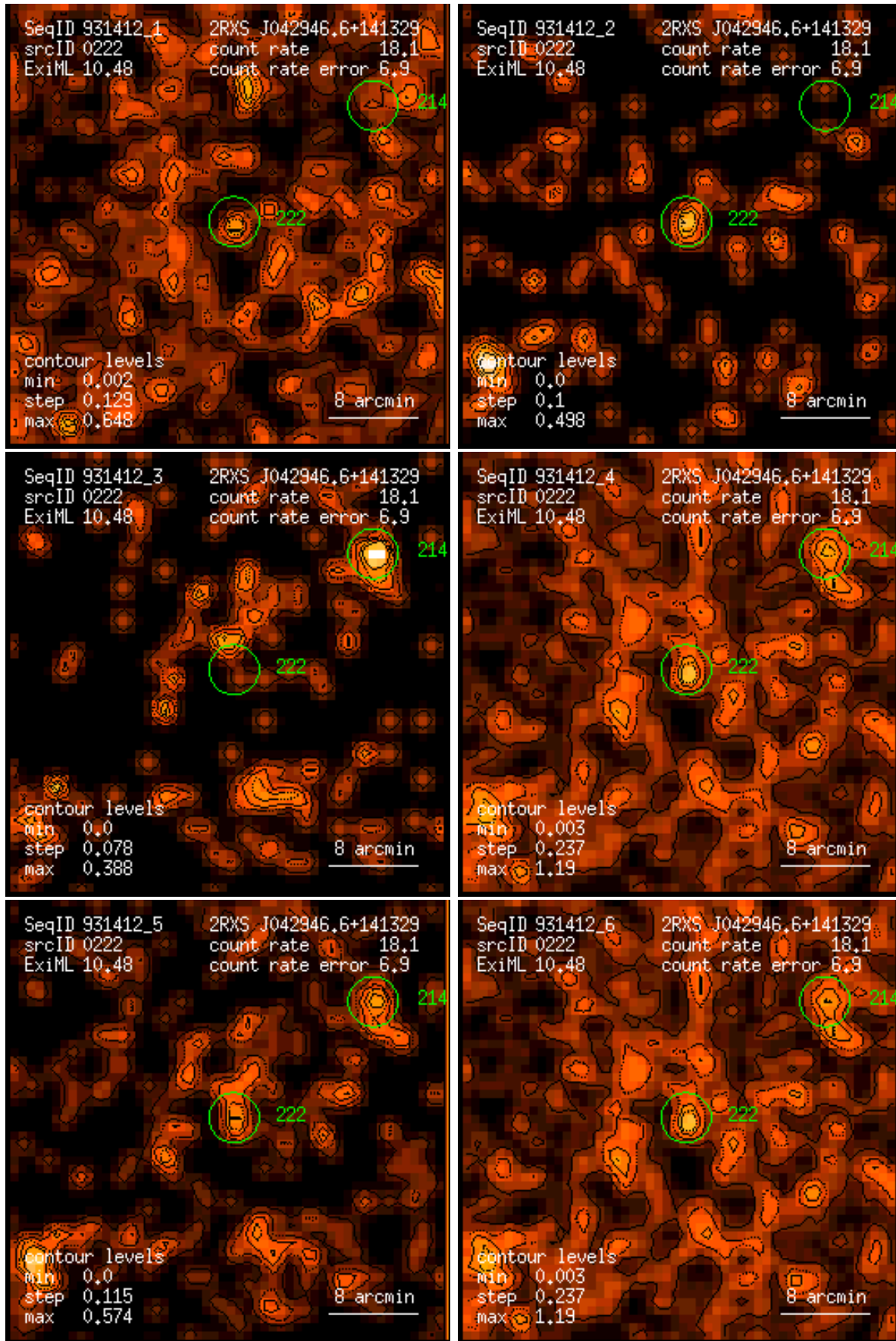
Figure 222: RASS 931412: detection 0222: band rate images, Gaussian filter: (1) PSPC channels 11 – 41, (2) 52 – 90, (3) 91 – 201, (4) 11 – 235, (5) 52 – 201, (6) 11 – 201. Broad band rates in counts/ks. Band rate contour levels in counts/ks/arcmin 2 .
