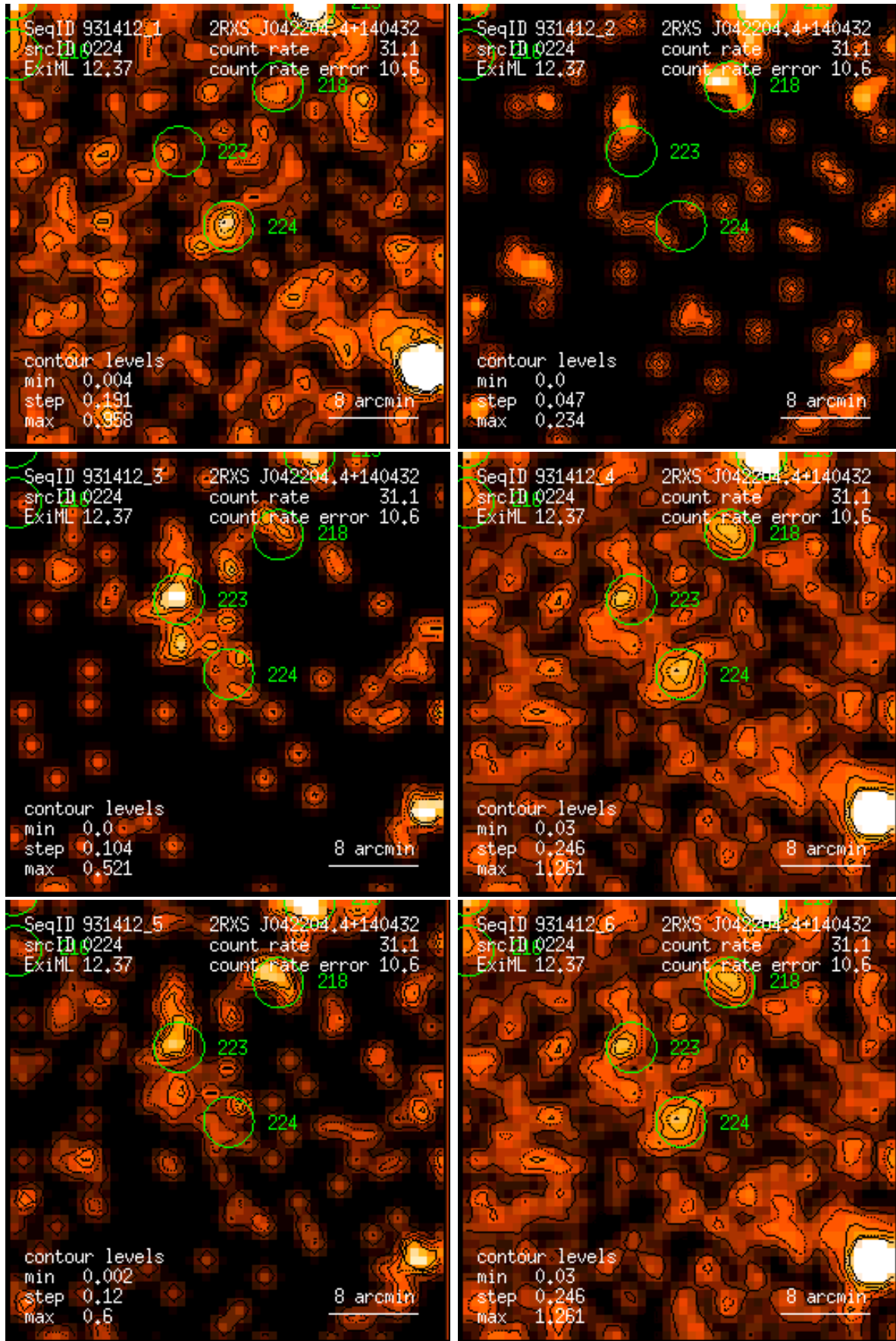
Figure 224: RASS 931412: detection 0224: band rate images, Gaussian filter: (1) PSPC channels 11 – 41, (2) 52 – 90, (3) 91 – 201, (4) 11 – 235, (5) 52 – 201, (6) 11 – 201. Broad band rates in counts/ks. Band rate contour levels in counts/ks/arcmin 2 .
