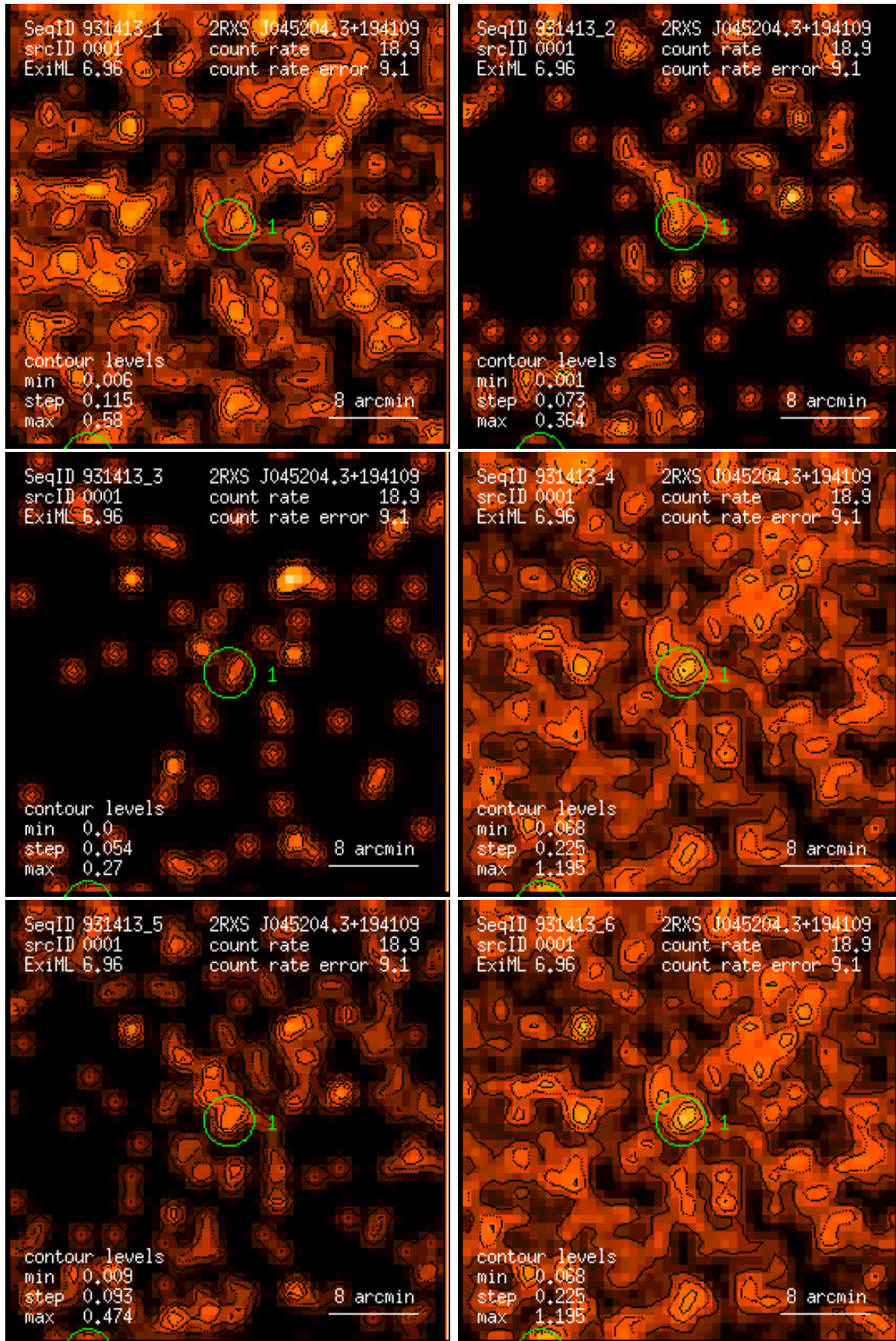
Figure 1: RASS 931413: detection 0001: band rate images, Gaussian filter: (1) PSPC channels 11 – 41, (2) 52 – 90, (3) 91 – 201, (4) 11 – 235, (5) 52 – 201, (6) 11 – 201. Broad band rates in counts/ks. Band rate contour levels in counts/ks/arcmin 2 .
