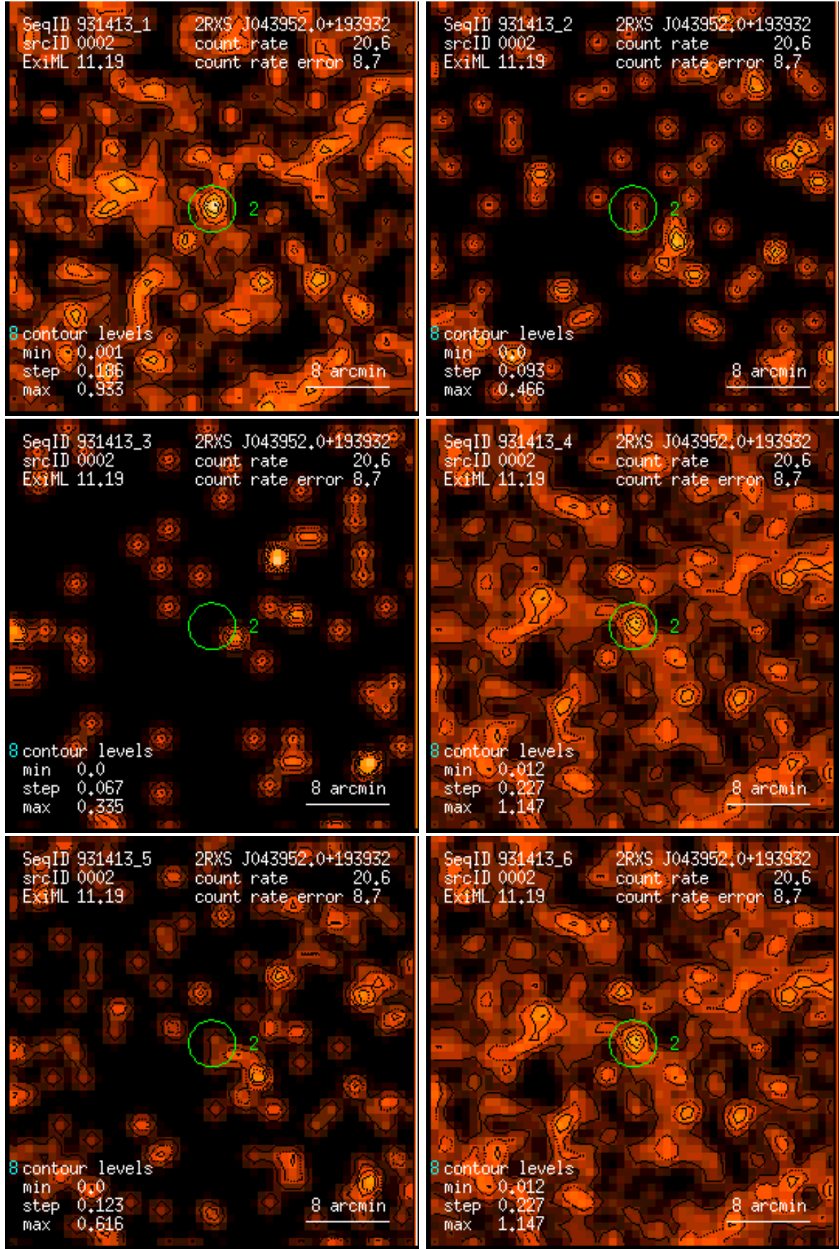
Figure 2: RASS 931413: detection 0002: band rate images, Gaussian filter: (1) PSPC channels 11 – 41, (2) 52 – 90, (3) 91 – 201, (4) 11 – 235, (5) 52 – 201, (6) 11 – 201. Broad band rates in counts/ks. Band rate contour levels in counts/ks/arcmin 2 .
