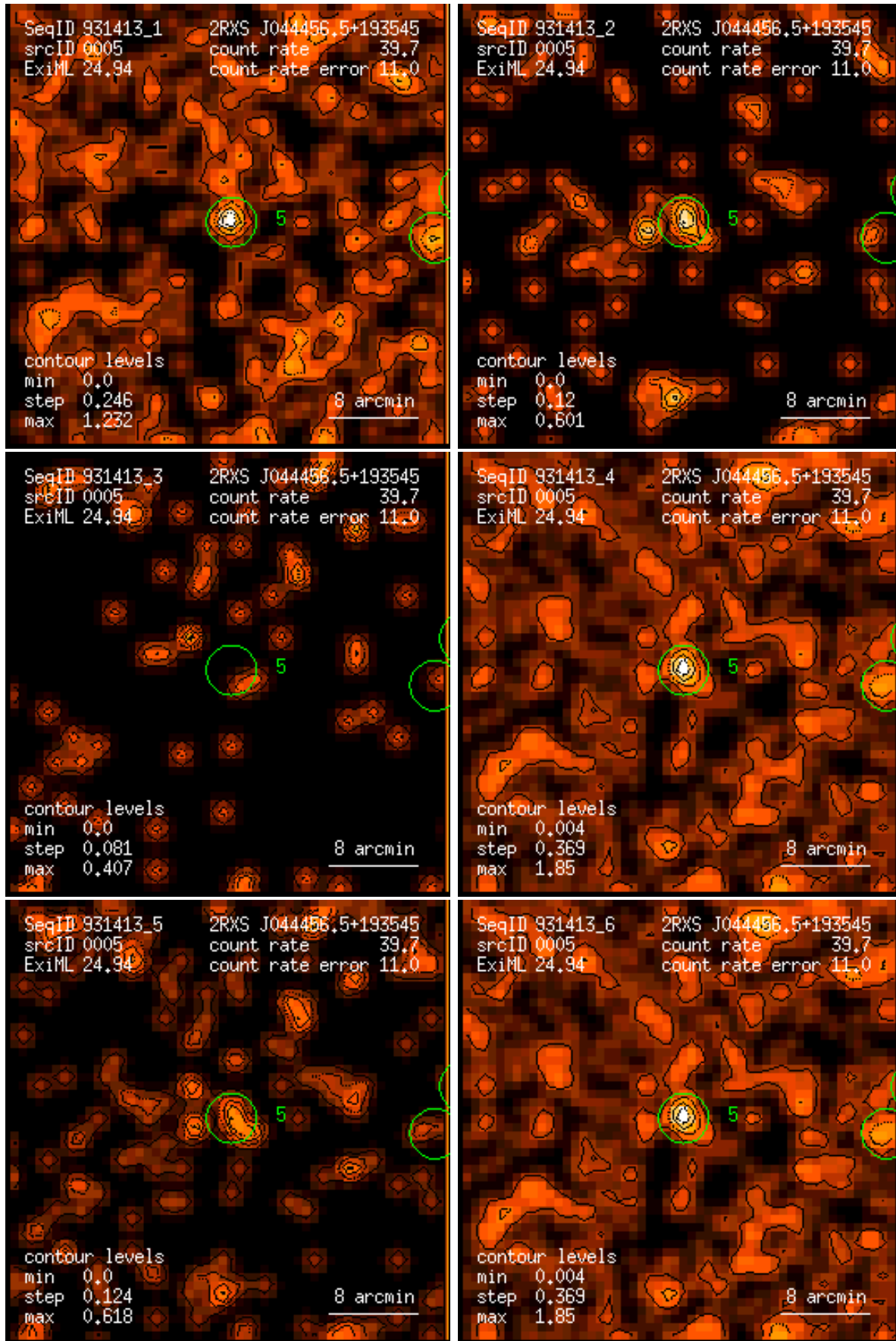
Figure 5: RASS 931413: detection 0005: band rate images, Gaussian filter: (1) PSPC channels 11 – 41, (2) 52 – 90, (3) 91 – 201, (4) 11 – 235, (5) 52 – 201, (6) 11 – 201. Broad band rates in counts/ks. Band rate contour levels in counts/ks/arcmin 2 .
