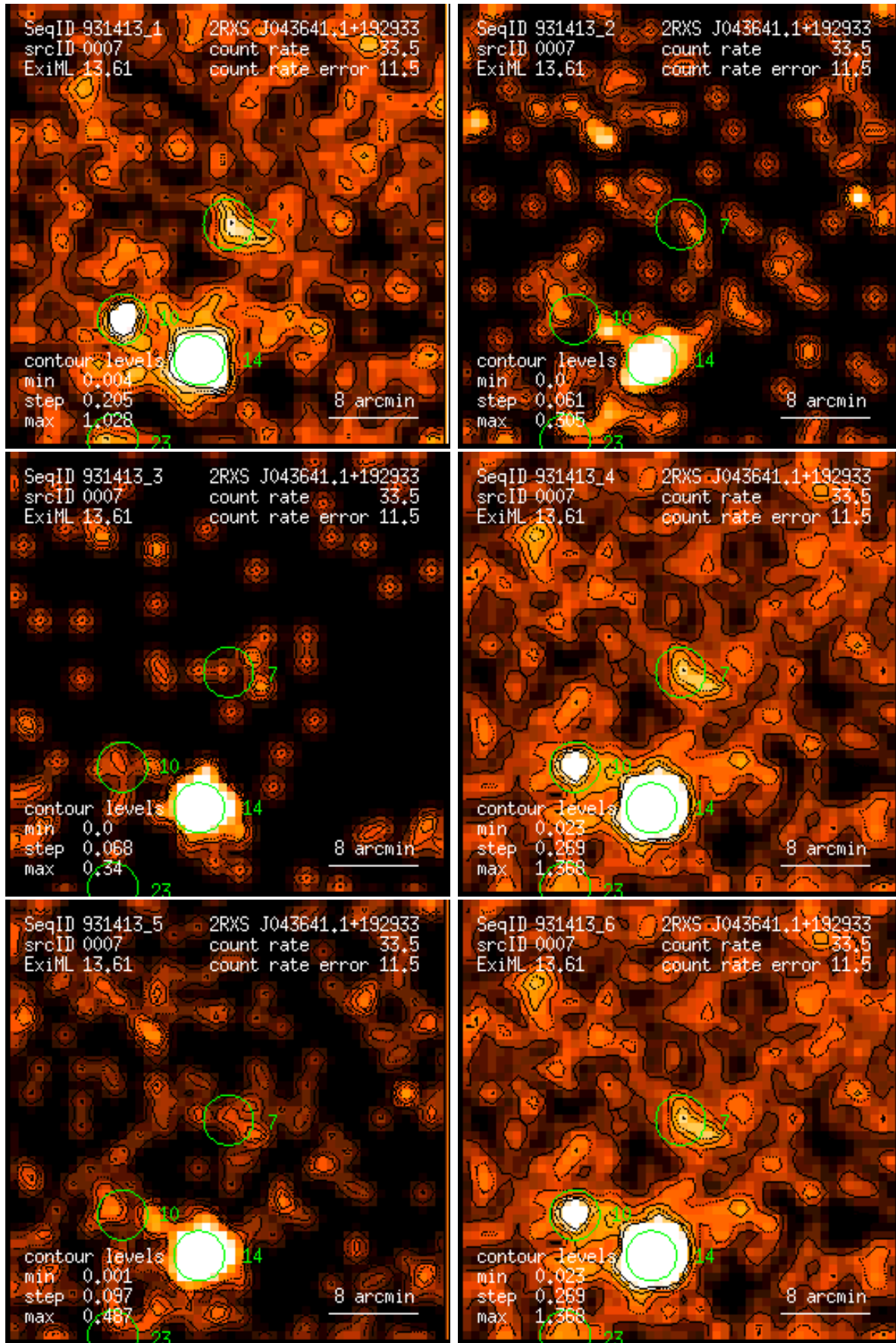
Figure 7: RASS 931413: detection 0007: band rate images, Gaussian filter: (1) PSPC channels 11 – 41, (2) 52 – 90, (3) 91 – 201, (4) 11 – 235, (5) 52 – 201, (6) 11 – 201. Broad band rates in counts/ks. Band rate contour levels in counts/ks/arcmin 2 .
