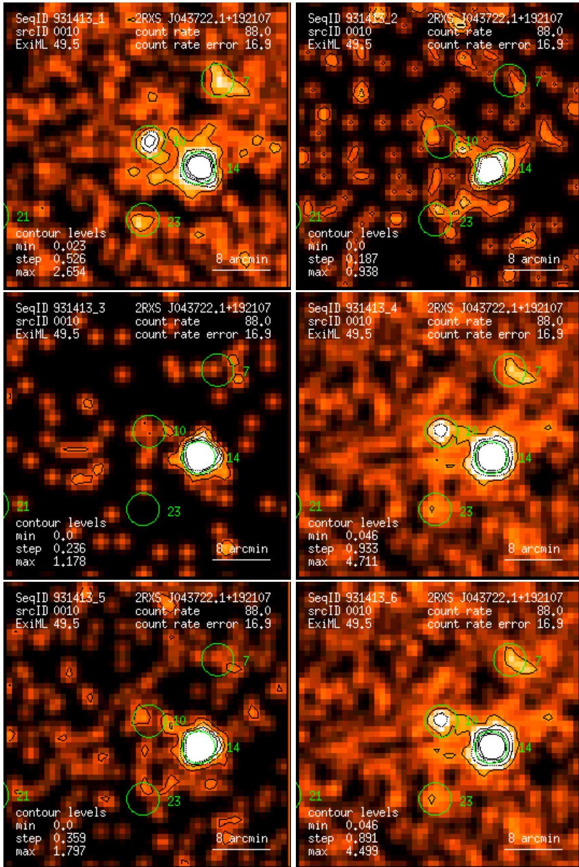
Figure 10: RASS 931413: detection 0010: band rate images, Gaussian filter: (1) PSPC channels 11 – 41, (2) 52 – 90, (3) 91 – 201, (4) 11 – 235, (5) 52 – 201, (6) 11 – 201. Broad band rates in counts/ks. Band rate contour levels in counts/ks/arcmin 2 .
