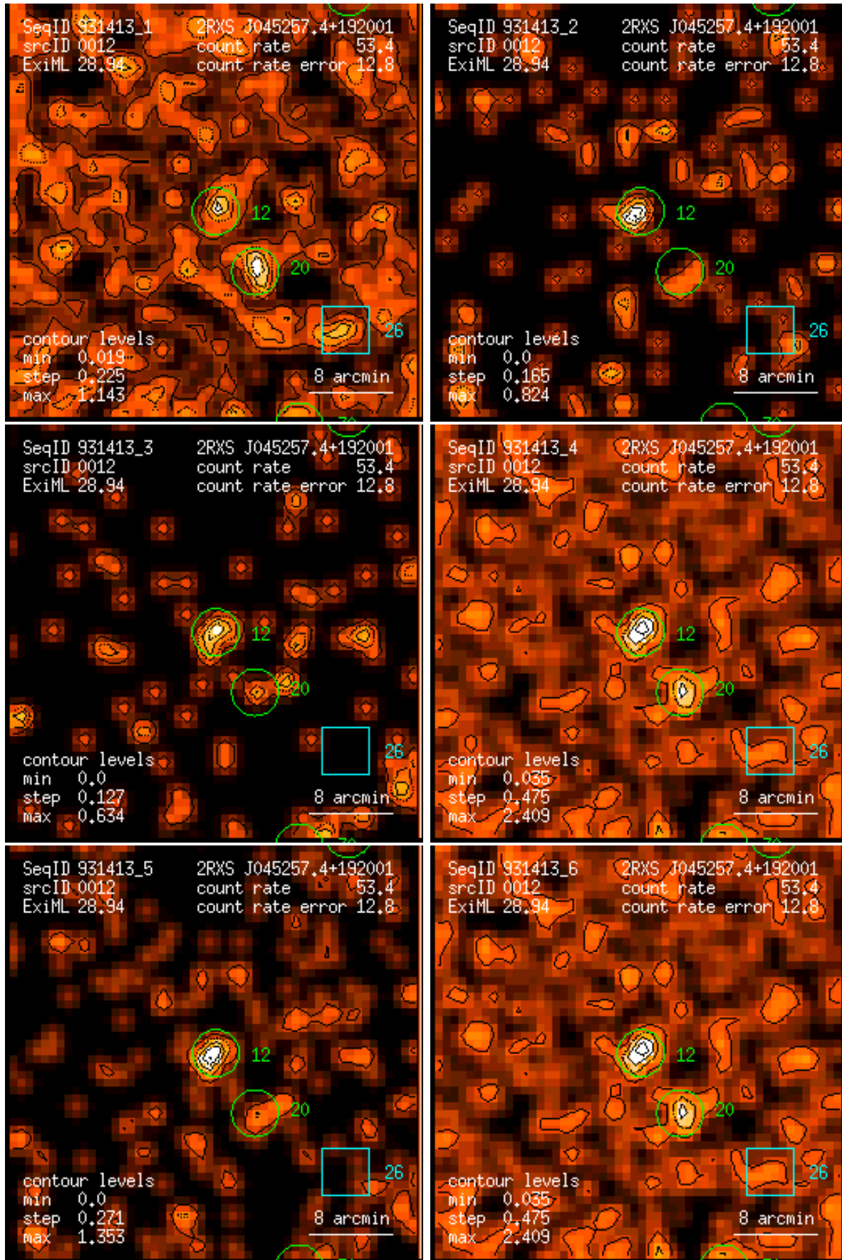
Figure 12: RASS 931413: detection 0012: band rate images, Gaussian filter: (1) PSPC channels 11 – 41, (2) 52 – 90, (3) 91 – 201, (4) 11 – 235, (5) 52 – 201, (6) 11 – 201. Broad band rates in counts/ks. Band rate contour levels in counts/ks/arcmin 2 .
