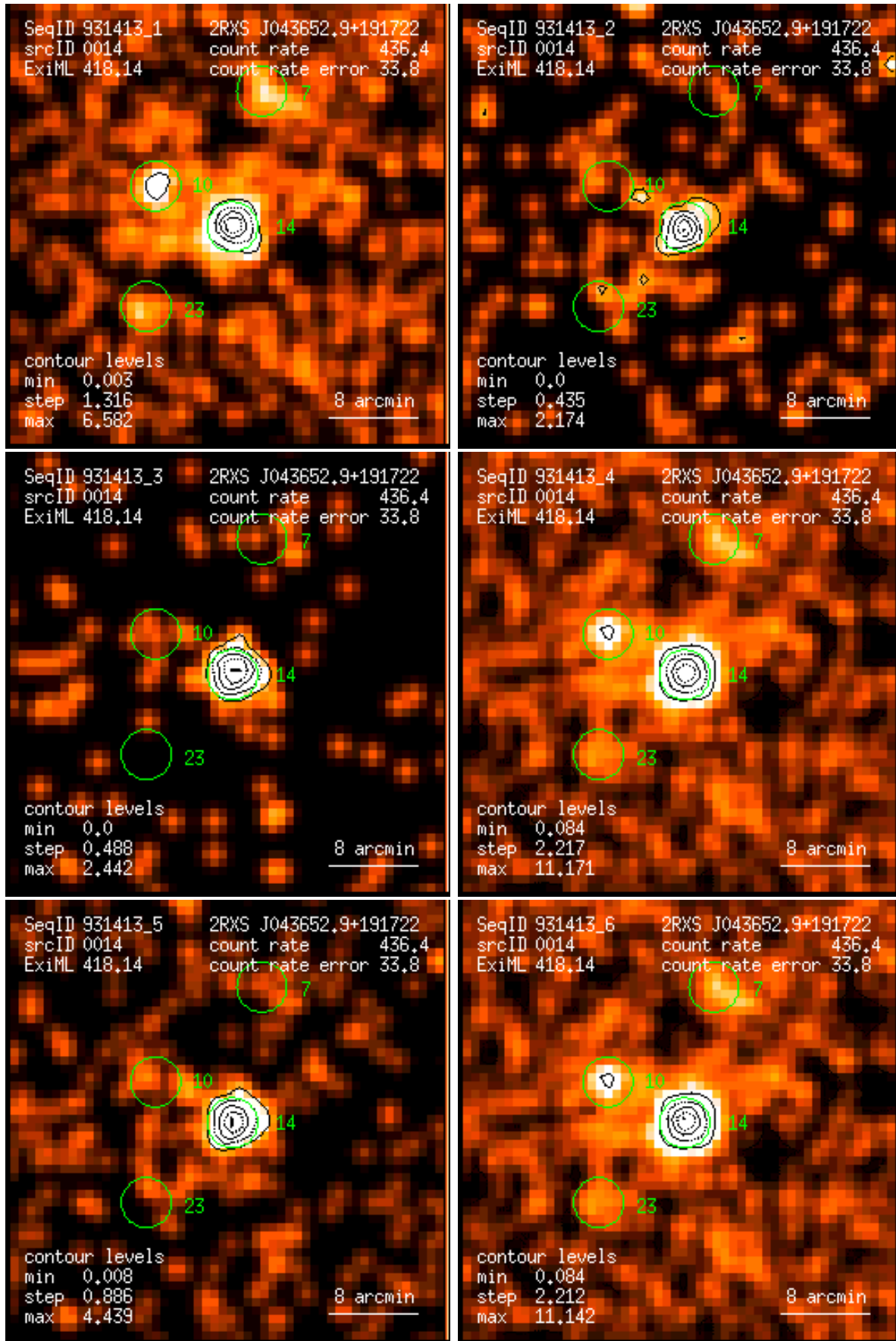
Figure 14: RASS 931413: detection 0014: band rate images, Gaussian filter: (1) PSPC channels 11 – 41, (2) 52 – 90, (3) 91 – 201, (4) 11 – 235, (5) 52 – 201, (6) 11 – 201. Broad band rates in counts/ks. Band rate contour levels in counts/ks/arcmin 2 .
