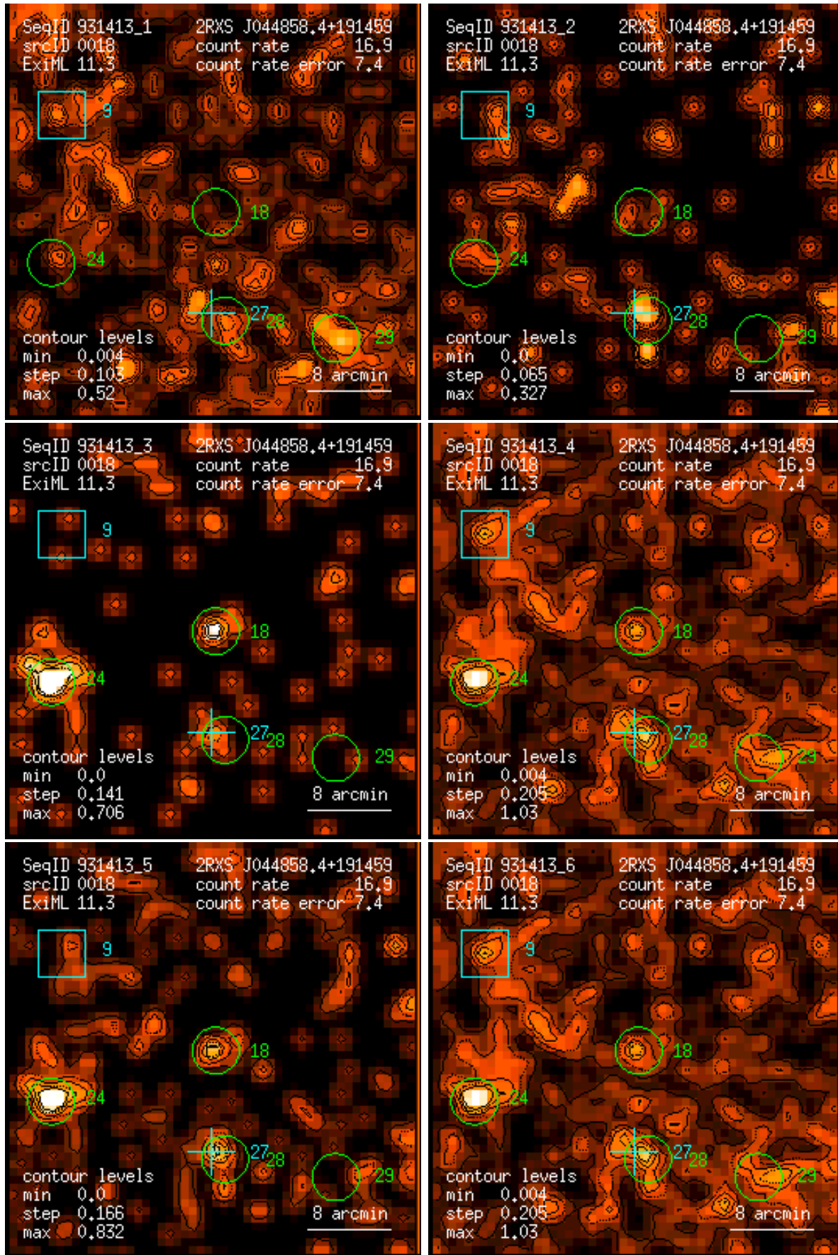
Figure 18: RASS 931413: detection 0018: band rate images, Gaussian filter: (1) PSPC channels 11 – 41, (2) 52 – 90, (3) 91 – 201, (4) 11 – 235, (5) 52 – 201, (6) 11 – 201. Broad band rates in counts/ks. Band rate contour levels in counts/ks/arcmin 2 .
