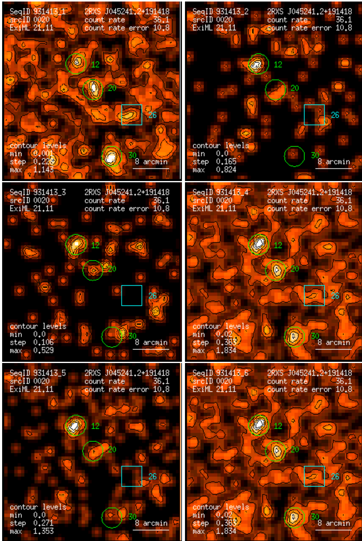
Figure 20: RASS 931413: detection 0020: band rate images, Gaussian filter: (1) PSPC channels 11 – 41, (2) 52 – 90, (3) 91 – 201, (4) 11 – 235, (5) 52 – 201, (6) 11 – 201. Broad band rates in counts/ks. Band rate contour levels in counts/ks/arcmin 2 .
