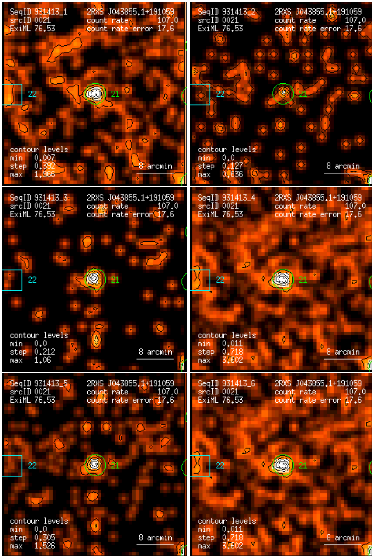
Figure 21: RASS 931413: detection 0021: band rate images, Gaussian filter: (1) PSPC channels 11 – 41, (2) 52 – 90, (3) 91 – 201, (4) 11 – 235, (5) 52 – 201, (6) 11 – 201. Broad band rates in counts/ks. Band rate contour levels in counts/ks/arcmin 2 .
